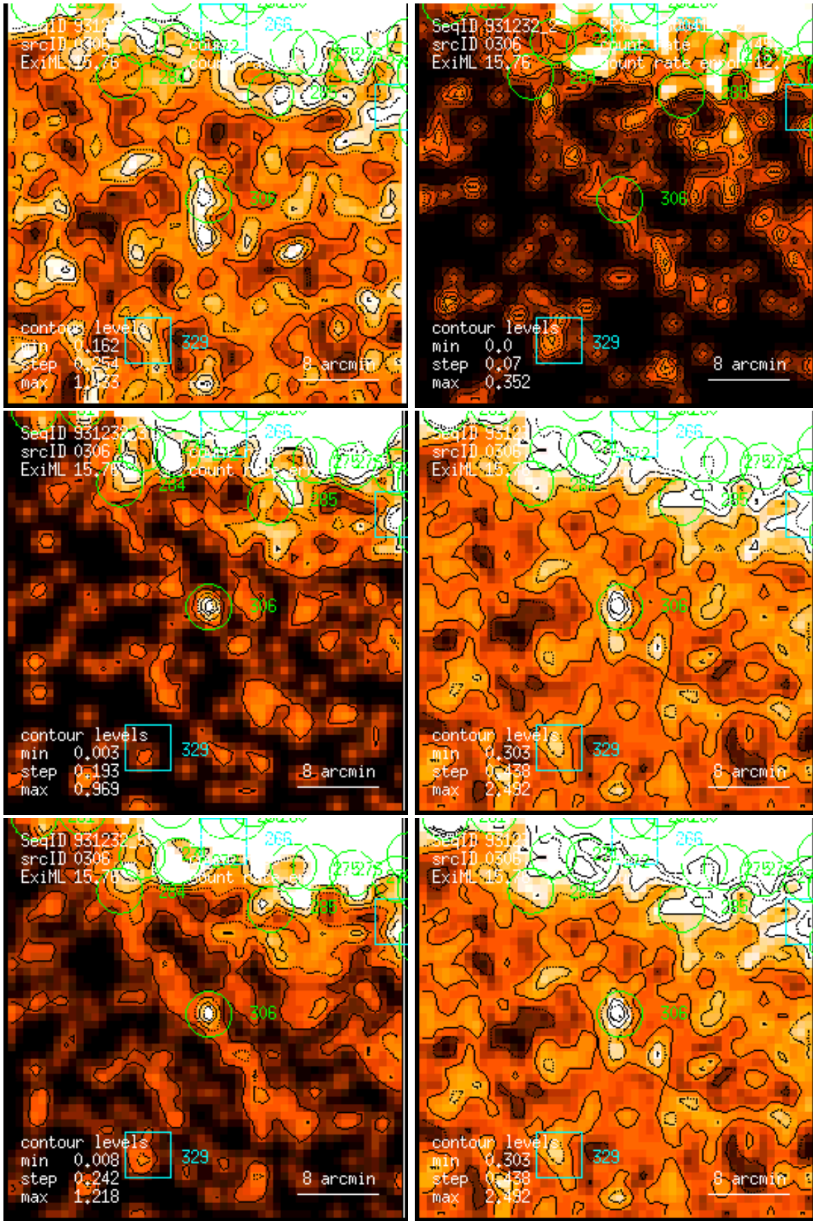
Figure 306: RASS 931232: detection 0306: band rate images, Gaussian filter: (1) PSPC channels 11 – 41, (2) 52 – 90, (3) 91 – 201, (4) 11 – 235, (5) 52 – 201, (6) 11 – 201. Broad band rates in counts/ks. Band rate contour levels in counts/ks/arcmin 2 .
