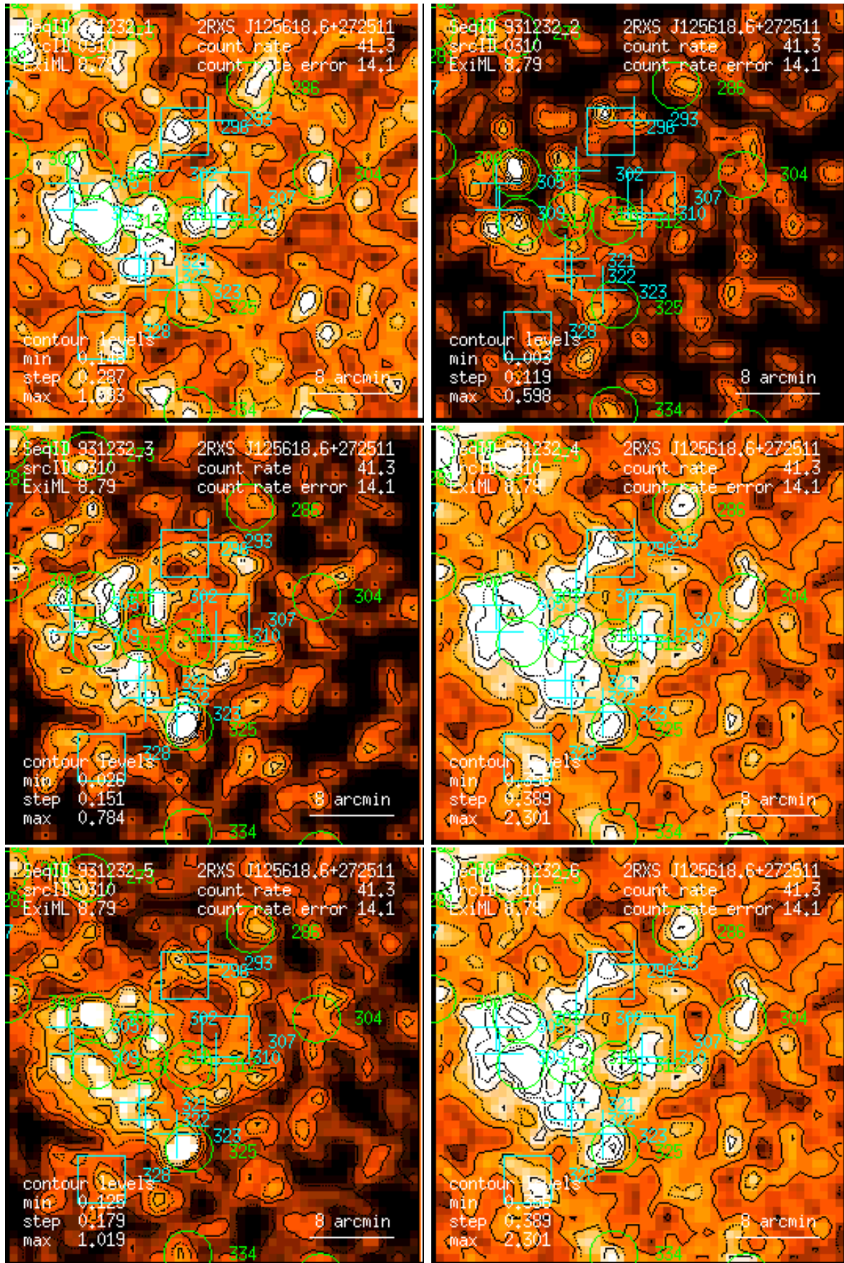
Figure 310: RASS 931232: detection 0310: band rate images, Gaussian filter: (1) PSPC channels 11 – 41, (2) 52 – 90, (3) 91 – 201, (4) 11 – 235, (5) 52 – 201, (6) 11 – 201. Broad band rates in counts/ks. Band rate contour levels in counts/ks/arcmin 2 .
