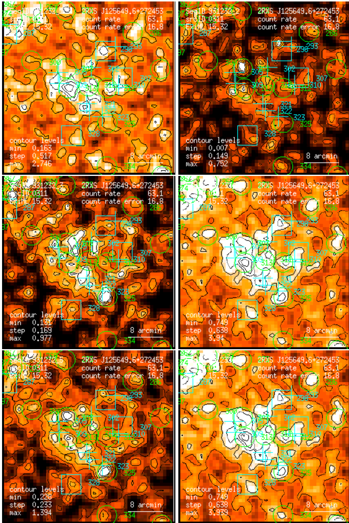
Figure 311: RASS 931232: detection 0311: band rate images, Gaussian filter: (1) PSPC channels 11 – 41, (2) 52 – 90, (3) 91 – 201, (4) 11 – 235, (5) 52 – 201, (6) 11 – 201. Broad band rates in counts/ks. Band rate contour levels in counts/ks/arcmin 2 .
