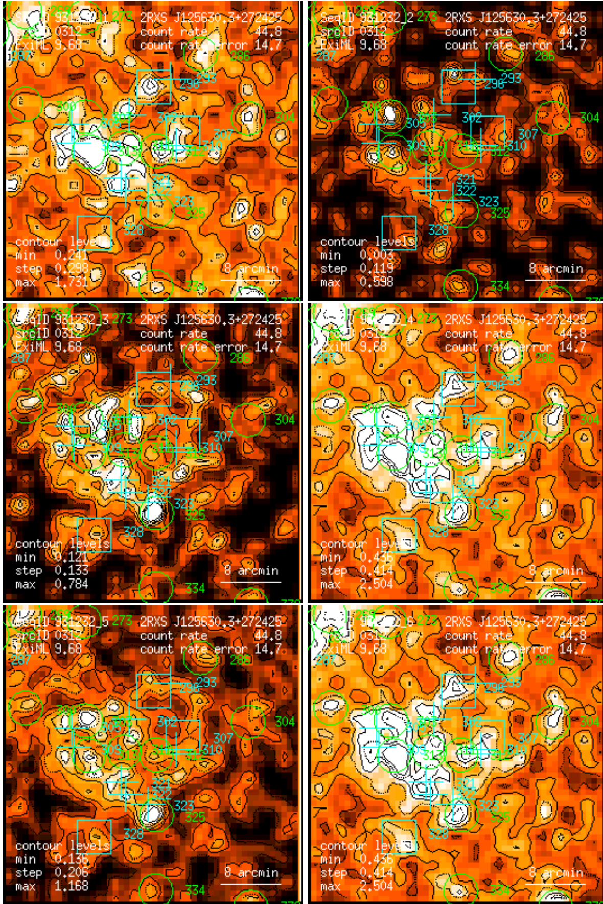
Figure 312: RASS 931232: detection 0312: band rate images, Gaussian filter: (1) PSPC channels 11 – 41, (2) 52 – 90, (3) 91 – 201, (4) 11 – 235, (5) 52 – 201, (6) 11 – 201. Broad band rates in counts/ks. Band rate contour levels in counts/ks/arcmin 2 .
