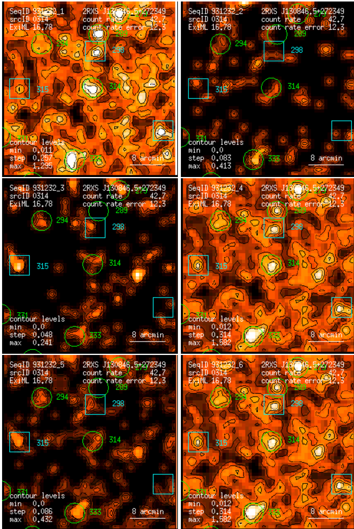
Figure 314: RASS 931232: detection 0314: band rate images, Gaussian filter: (1) PSPC channels 11 – 41, (2) 52 – 90, (3) 91 – 201, (4) 11 – 235, (5) 52 – 201, (6) 11 – 201. Broad band rates in counts/ks. Band rate contour levels in counts/ks/arcmin 2 .
