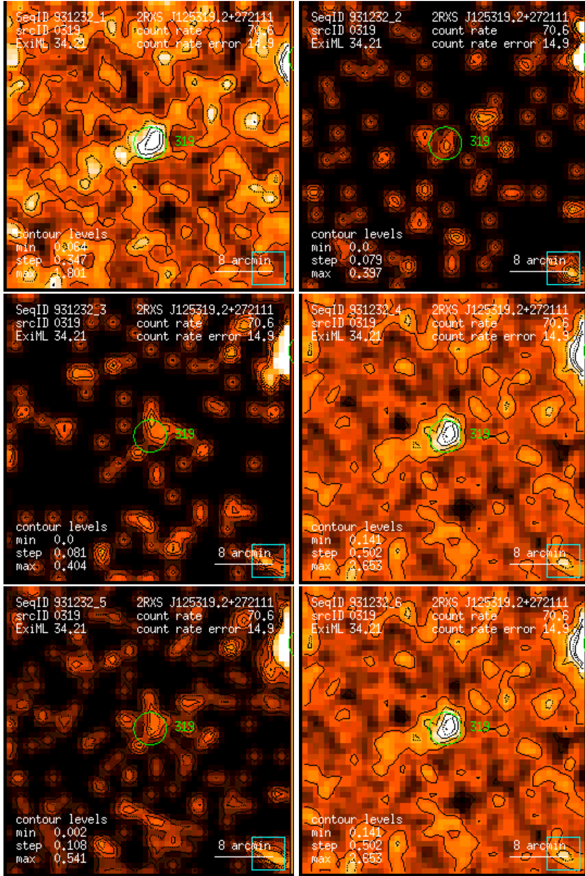
Figure 319: RASS 931232: detection 0319: band rate images, Gaussian filter: (1) PSPC channels 11 – 41, (2) 52 – 90, (3) 91 – 201, (4) 11 – 235, (5) 52 – 201, (6) 11 – 201. Broad band rates in counts/ks. Band rate contour levels in counts/ks/arcmin 2 .
