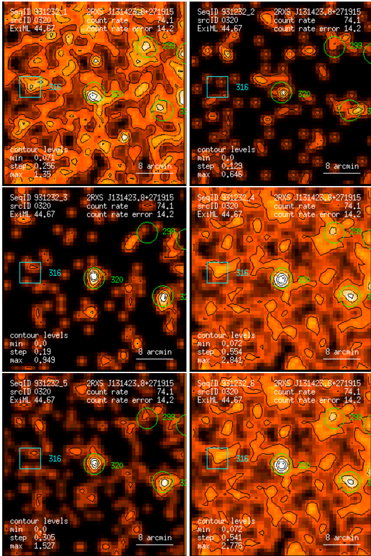
Figure 320: RASS 931232: detection 0320: band rate images, Gaussian filter: (1) PSPC channels 11 – 41, (2) 52 – 90, (3) 91 – 201, (4) 11 – 235, (5) 52 – 201, (6) 11 – 201. Broad band rates in counts/ks. Band rate contour levels in counts/ks/arcmin 2 .
