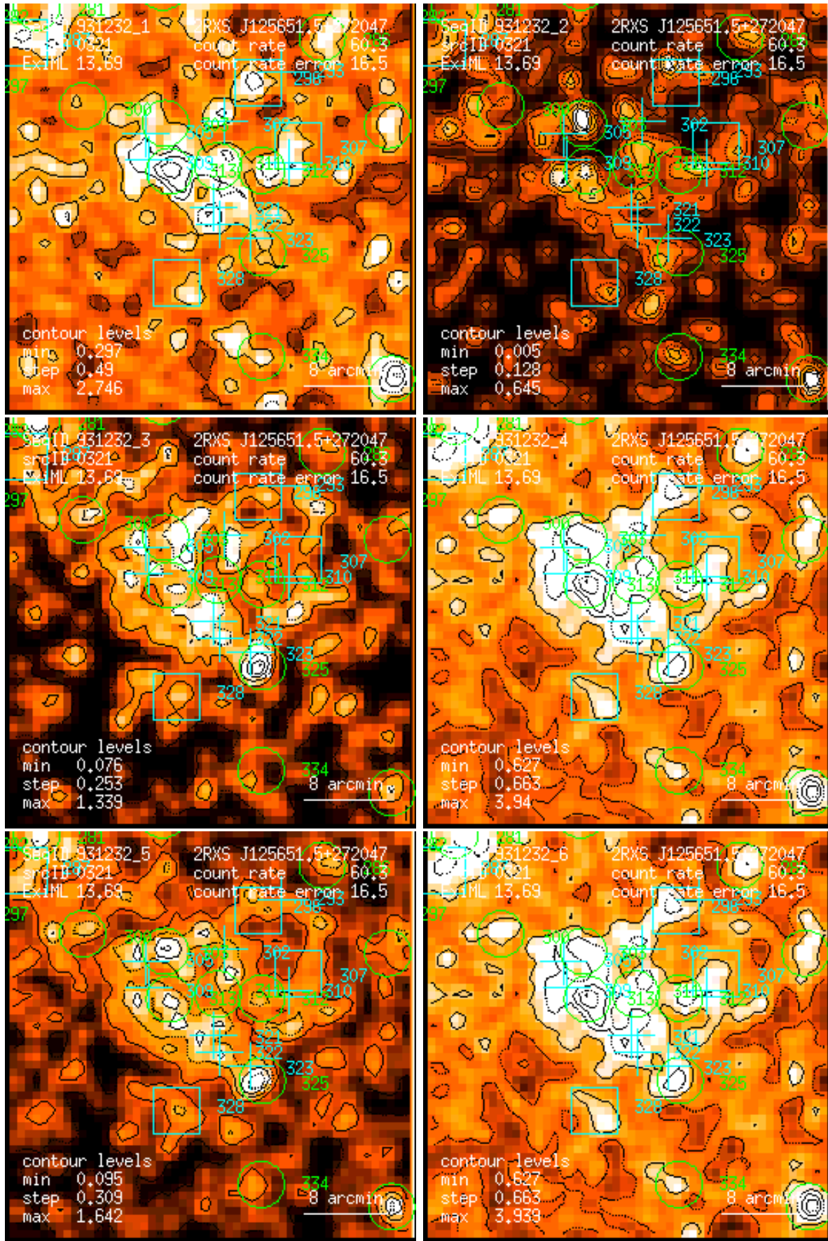
Figure 321: RASS 931232: detection 0321: band rate images, Gaussian filter: (1) PSPC channels 11 – 41, (2) 52 – 90, (3) 91 – 201, (4) 11 – 235, (5) 52 – 201, (6) 11 – 201. Broad band rates in counts/ks. Band rate contour levels in counts/ks/arcmin 2 .
