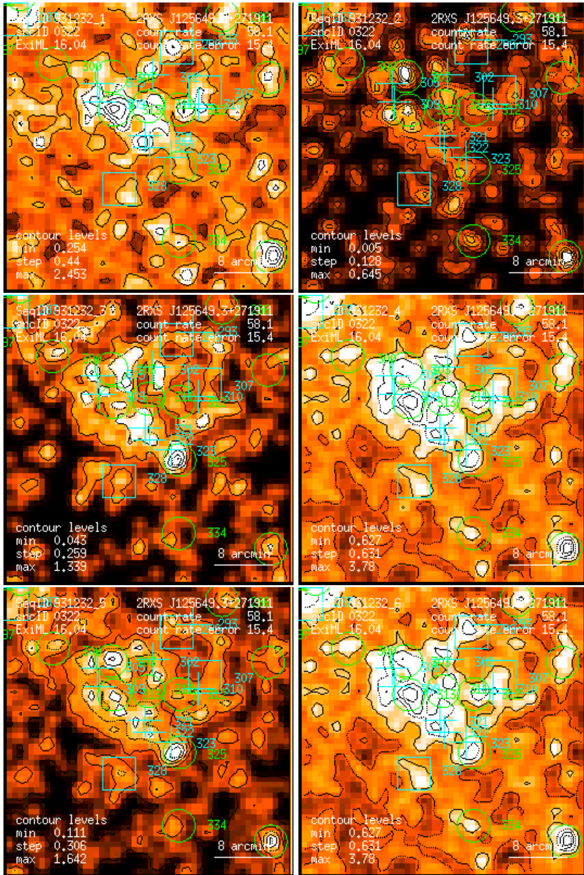
Figure 322: RASS 931232: detection 0322: band rate images, Gaussian filter: (1) PSPC channels 11 – 41, (2) 52 – 90, (3) 91 – 201, (4) 11 – 235, (5) 52 – 201, (6) 11 – 201. Broad band rates in counts/ks. Band rate contour levels in counts/ks/arcmin 2 .
