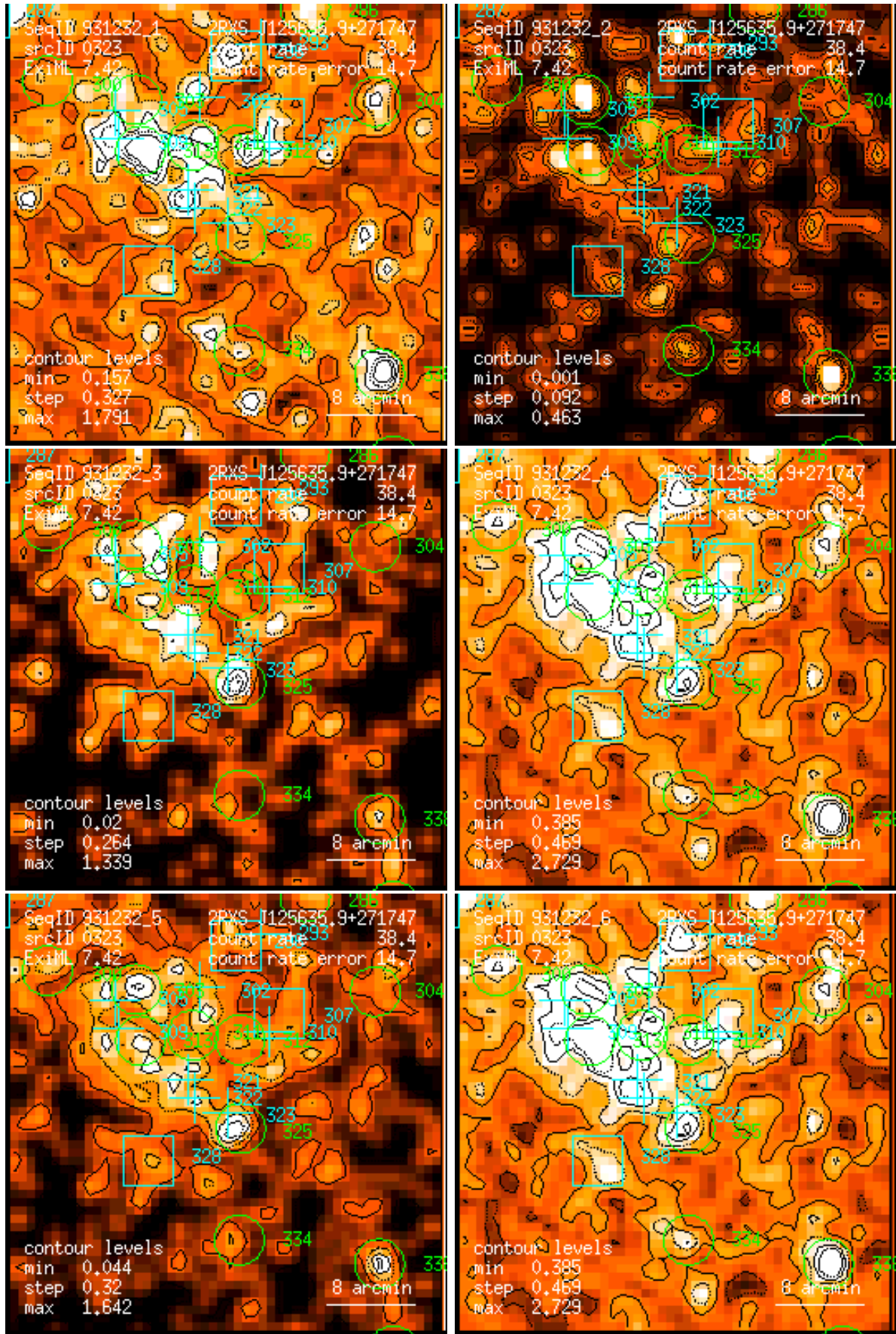
Figure 323: RASS 931232: detection 0323: band rate images, Gaussian filter: (1) PSPC channels 11 – 41, (2) 52 – 90, (3) 91 – 201, (4) 11 – 235, (5) 52 – 201, (6) 11 – 201. Broad band rates in counts/ks. Band rate contour levels in counts/ks/arcmin 2 .
