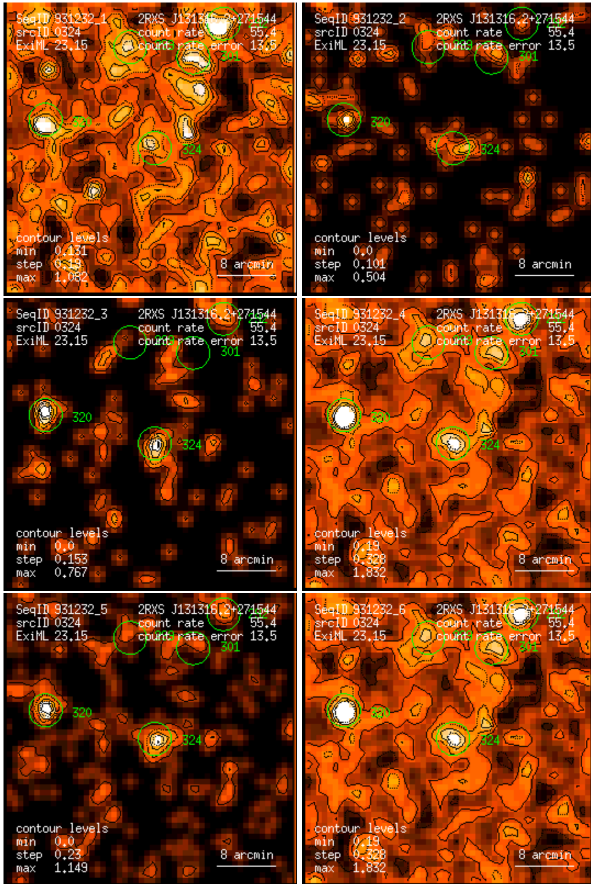
Figure 324: RASS 931232: detection 0324: band rate images, Gaussian filter: (1) PSPC channels 11 – 41, (2) 52 – 90, (3) 91 – 201, (4) 11 – 235, (5) 52 – 201, (6) 11 – 201. Broad band rates in counts/ks. Band rate contour levels in counts/ks/arcmin 2 .
