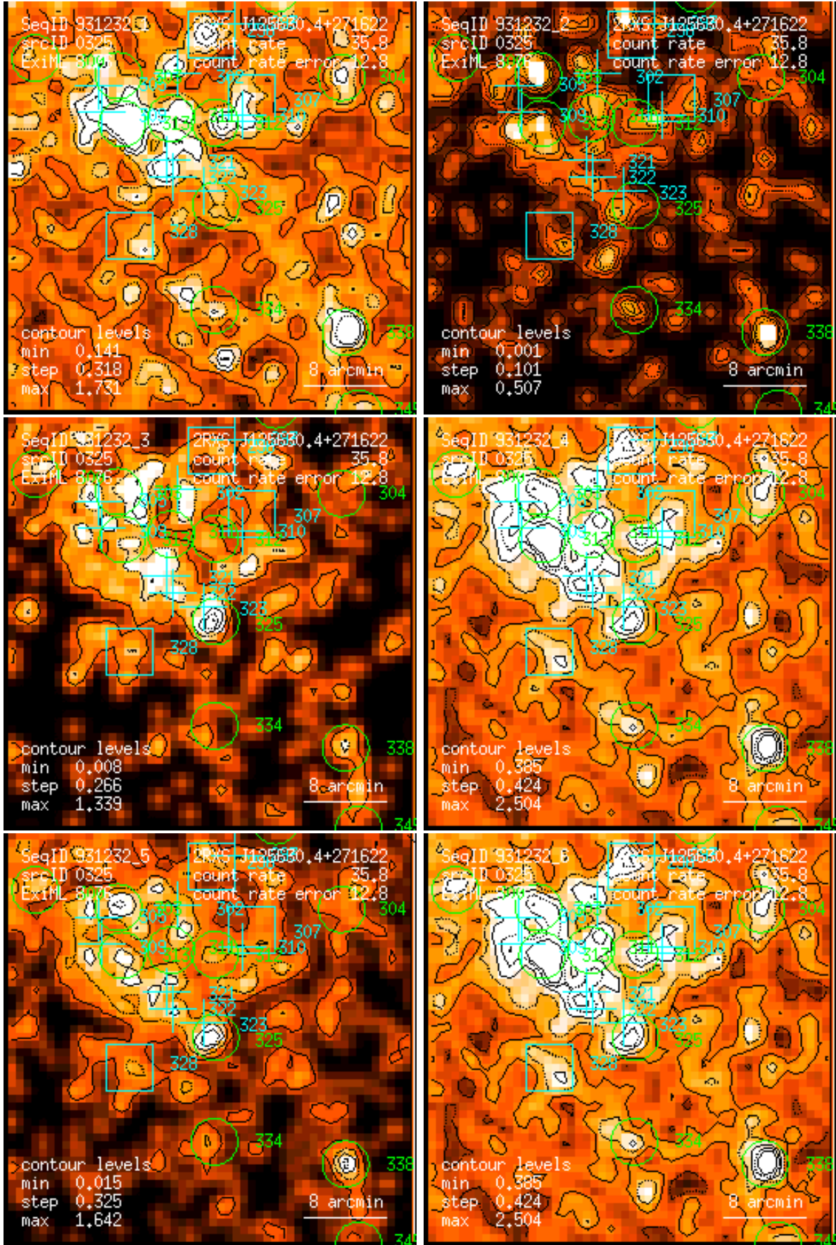
Figure 325: RASS 931232: detection 0325: band rate images, Gaussian filter: (1) PSPC channels 11 – 41, (2) 52 – 90, (3) 91 – 201, (4) 11 – 235, (5) 52 – 201, (6) 11 – 201. Broad band rates in counts/ks. Band rate contour levels in counts/ks/arcmin 2 .
