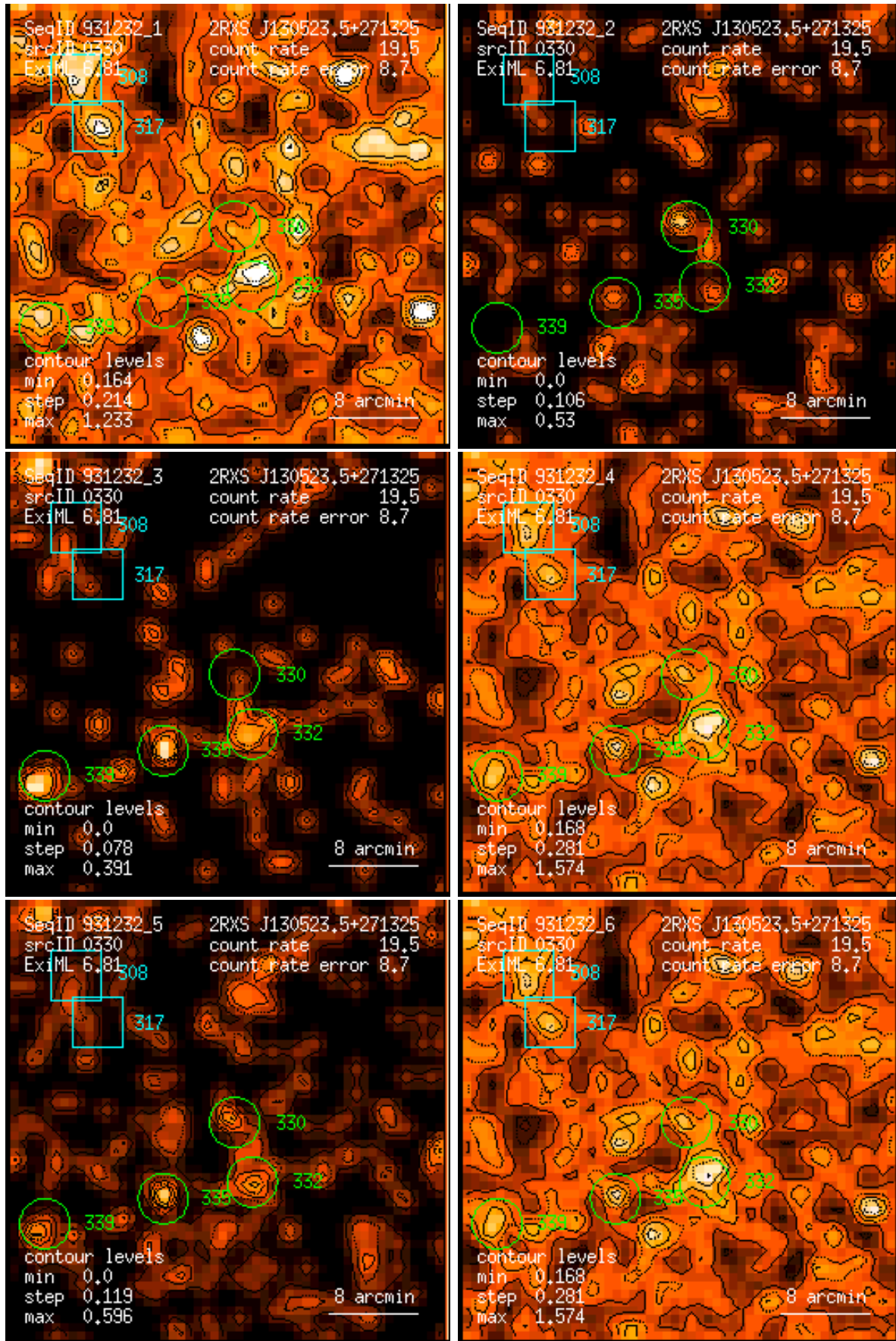
Figure 330: RASS 931232: detection 0330: band rate images, Gaussian filter: (1) PSPC channels 11 – 41, (2) 52 – 90, (3) 91 – 201, (4) 11 – 235, (5) 52 – 201, (6) 11 – 201. Broad band rates in counts/ks. Band rate contour levels in counts/ks/arcmin 2 .
