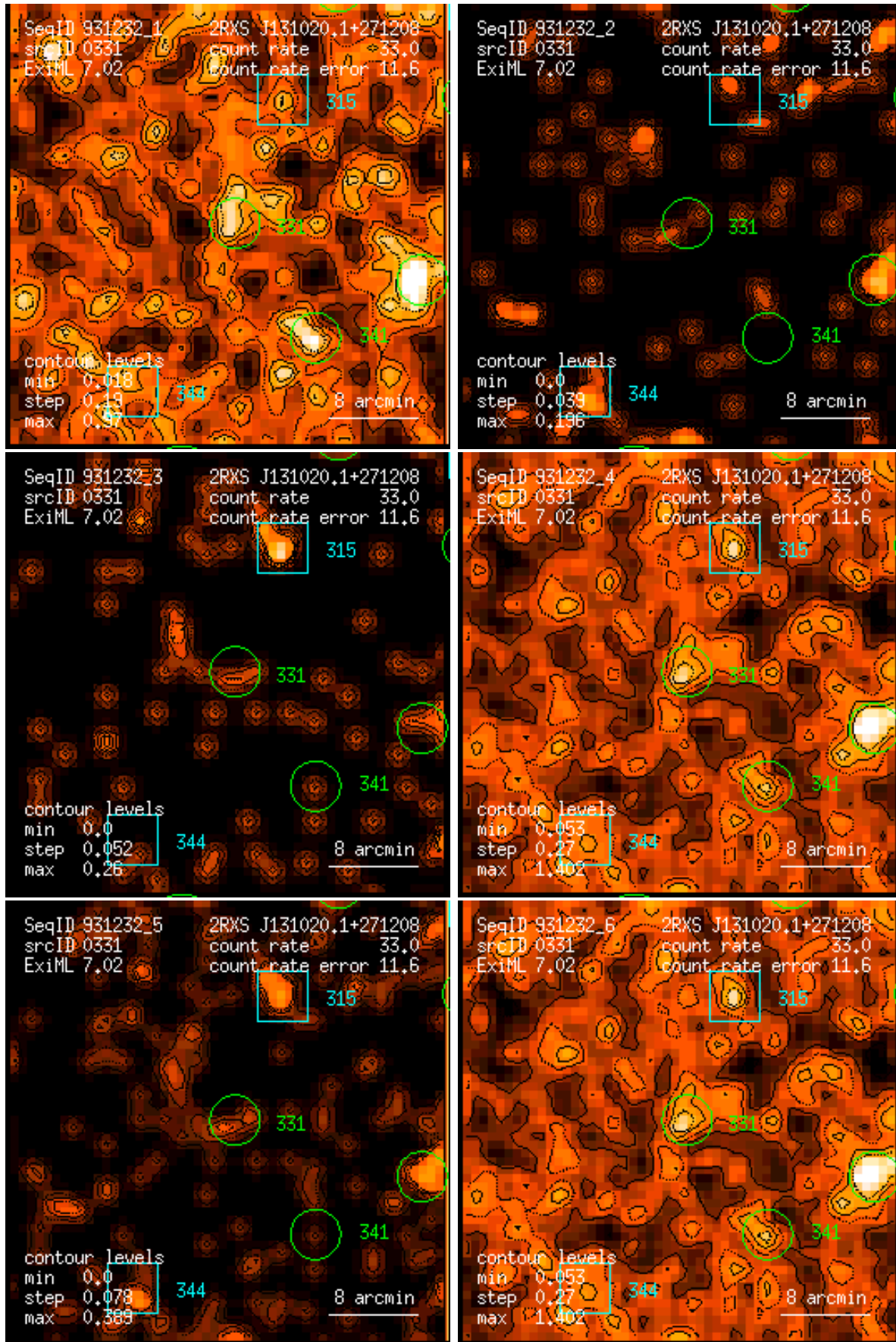
Figure 331: RASS 931232: detection 0331: band rate images, Gaussian filter: (1) PSPC channels 11 – 41, (2) 52 – 90, (3) 91 – 201, (4) 11 – 235, (5) 52 – 201, (6) 11 – 201. Broad band rates in counts/ks. Band rate contour levels in counts/ks/arcmin 2 .
