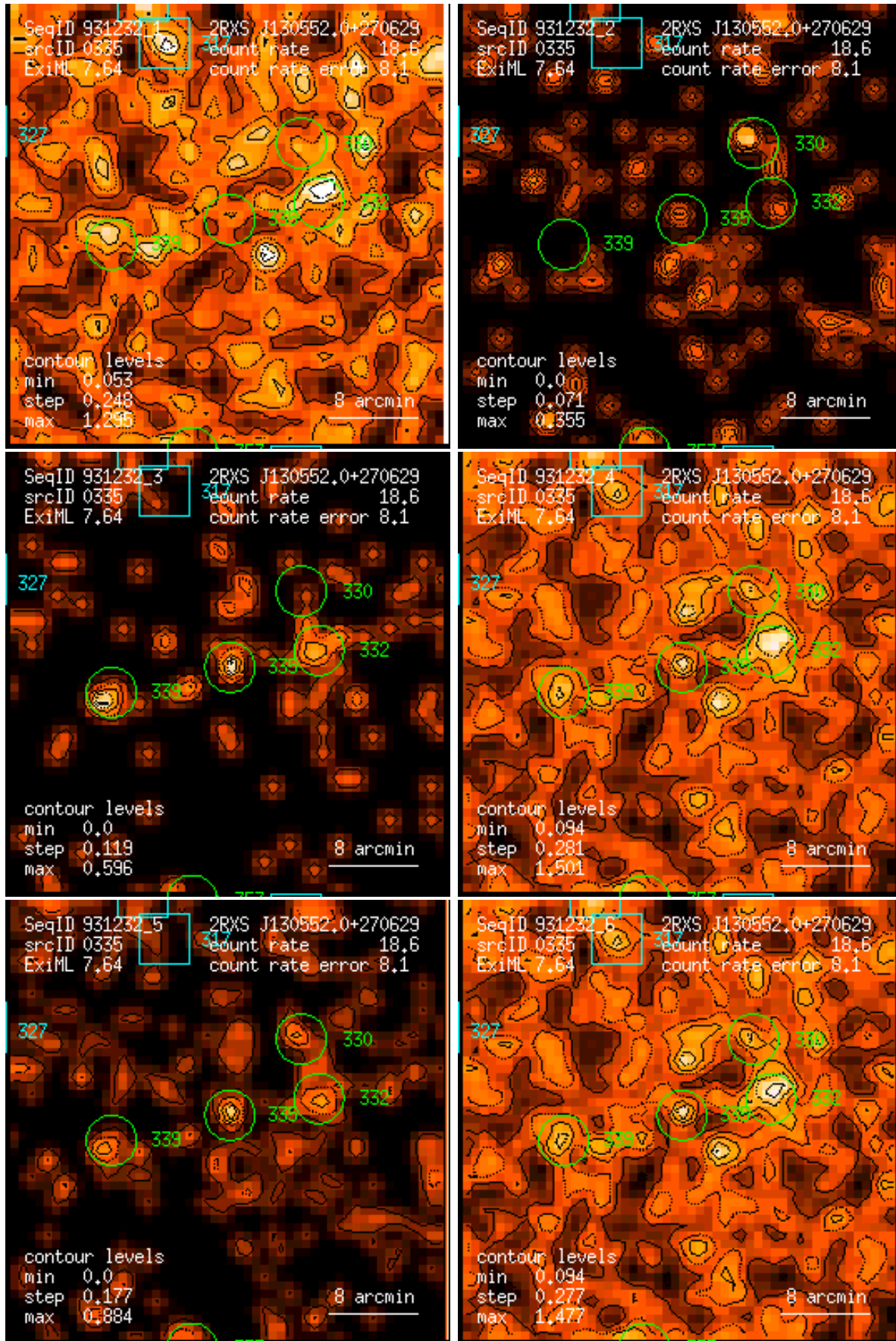
Figure 335: RASS 931232: detection 0335: band rate images, Gaussian filter: (1) PSPC channels 11 – 41, (2) 52 – 90, (3) 91 – 201, (4) 11 – 235, (5) 52 – 201, (6) 11 – 201. Broad band rates in counts/ks. Band rate contour levels in counts/ks/arcmin 2 .
