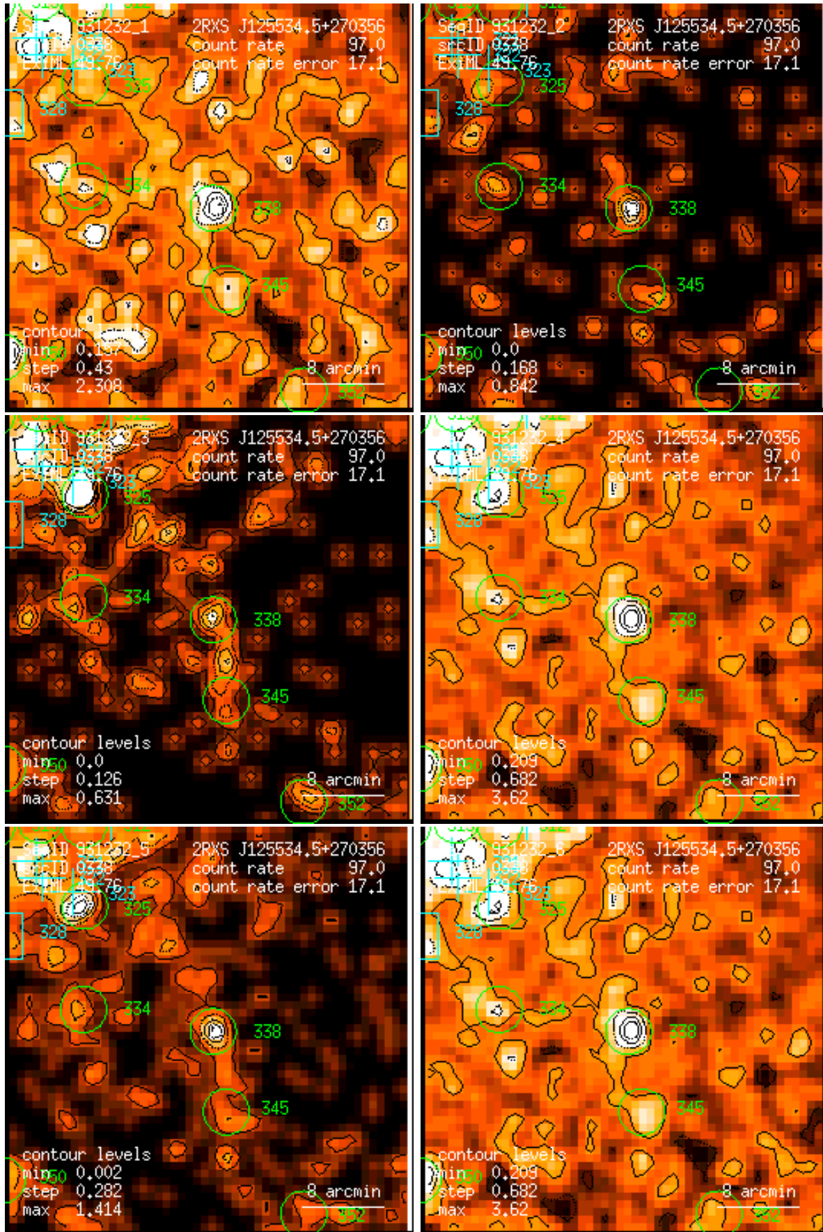
Figure 338: RASS 931232: detection 0338: band rate images, Gaussian filter: (1) PSPC channels 11 – 41, (2) 52 – 90, (3) 91 – 201, (4) 11 – 235, (5) 52 – 201, (6) 11 – 201. Broad band rates in counts/ks. Band rate contour levels in counts/ks/arcmin 2 .
