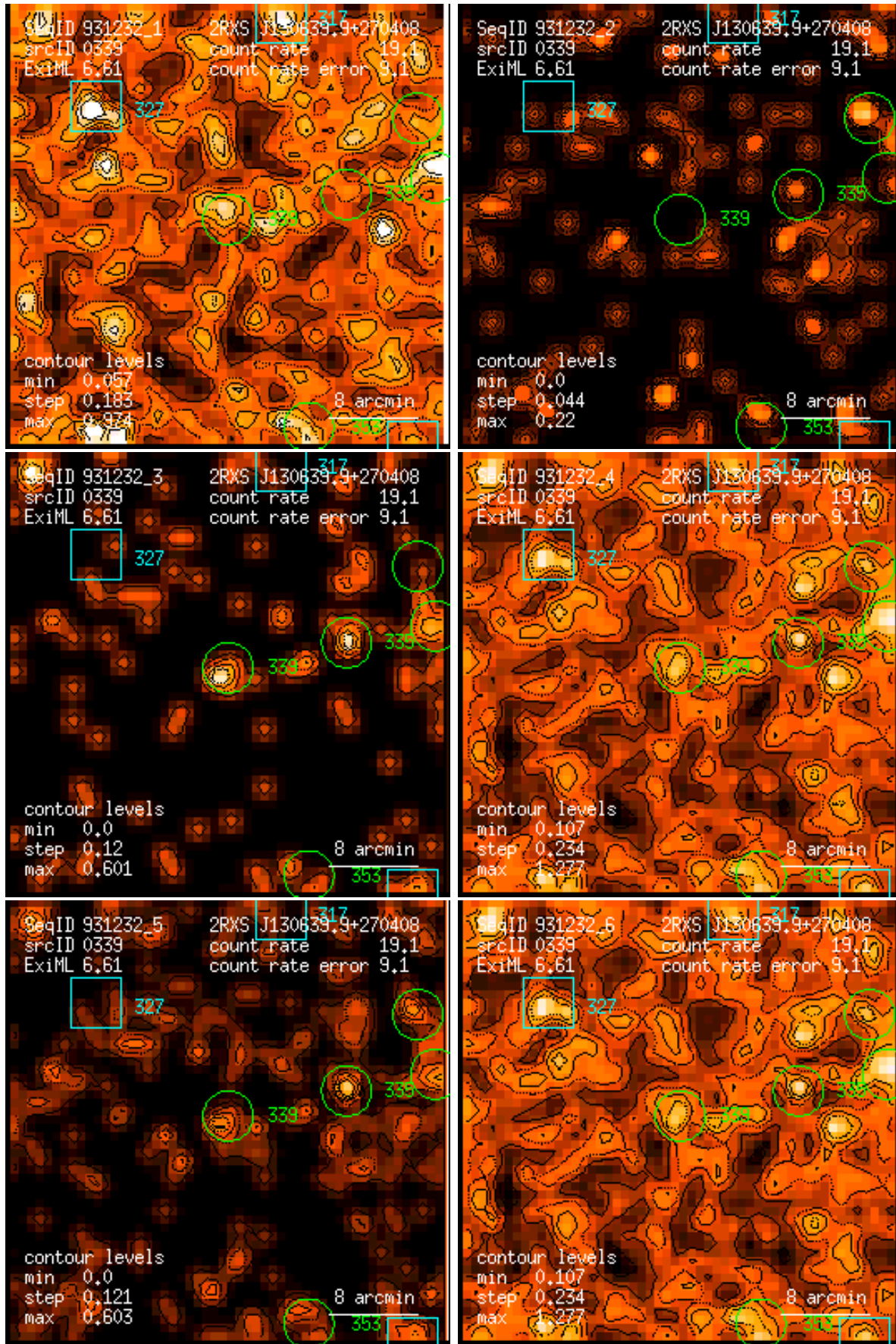
Figure 339: RASS 931232: detection 0339: band rate images, Gaussian filter: (1) PSPC channels 11 – 41, (2) 52 – 90, (3) 91 – 201, (4) 11 – 235, (5) 52 – 201, (6) 11 – 201. Broad band rates in counts/ks. Band rate contour levels in counts/ks/arcmin 2 .
