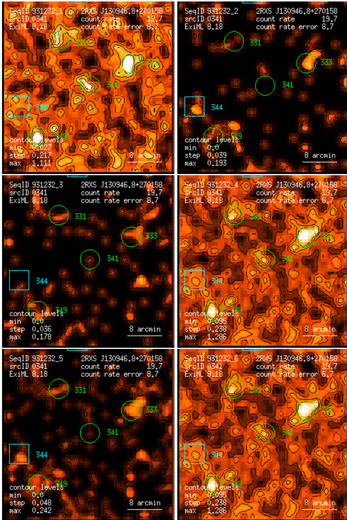
Figure 341: RASS 931232: detection 0341: band rate images, Gaussian filter: (1) PSPC channels 11 – 41, (2) 52 – 90, (3) 91 – 201, (4) 11 – 235, (5) 52 – 201, (6) 11 – 201. Broad band rates in counts/ks. Band rate contour levels in counts/ks/arcmin 2 .
