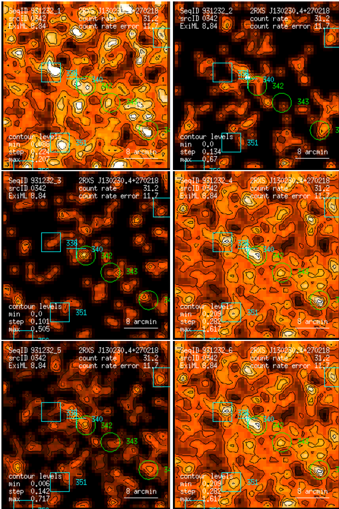
Figure 342: RASS 931232: detection 0342: band rate images, Gaussian filter: (1) PSPC channels 11 – 41, (2) 52 – 90, (3) 91 – 201, (4) 11 – 235, (5) 52 – 201, (6) 11 – 201. Broad band rates in counts/ks. Band rate contour levels in counts/ks/arcmin 2 .
