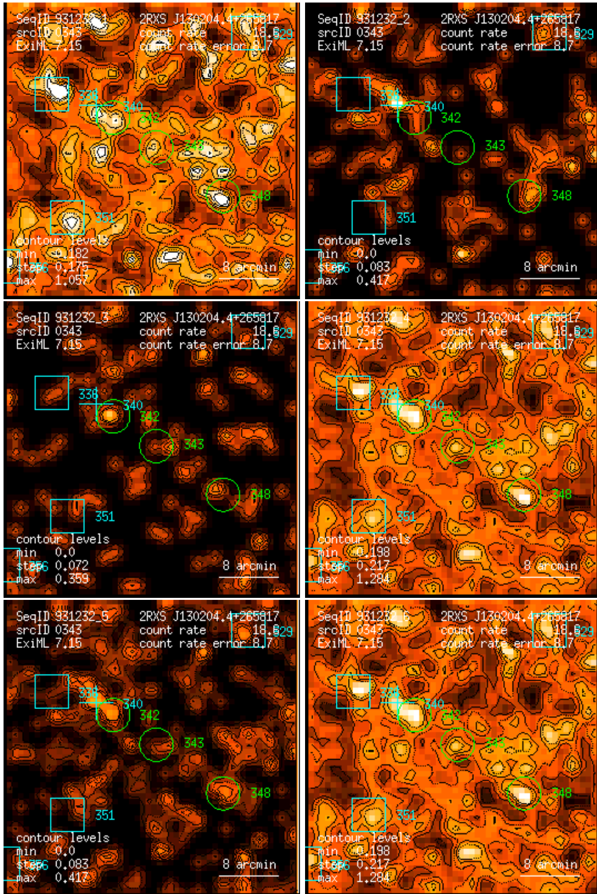
Figure 343: RASS 931232: detection 0343: band rate images, Gaussian filter: (1) PSPC channels 11 – 41, (2) 52 – 90, (3) 91 – 201, (4) 11 – 235, (5) 52 – 201, (6) 11 – 201. Broad band rates in counts/ks. Band rate contour levels in counts/ks/arcmin 2 .
