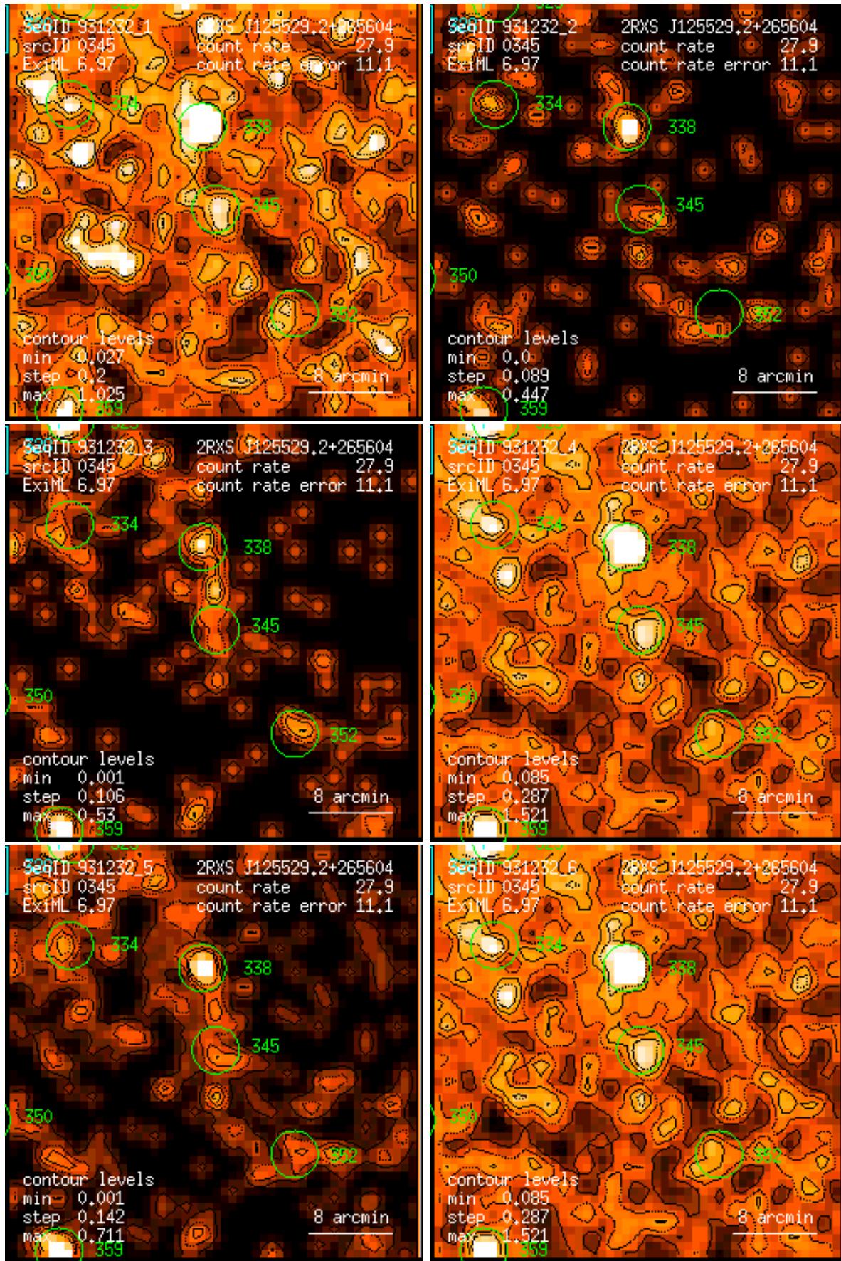
Figure 345: RASS 931232: detection 0345: band rate images, Gaussian filter: (1) PSPC channels 11 – 41, (2) 52 – 90, (3) 91 – 201, (4) 11 – 235, (5) 52 – 201, (6) 11 – 201. Broad band rates in counts/ks. Band rate contour levels in counts/ks/arcmin 2 .
