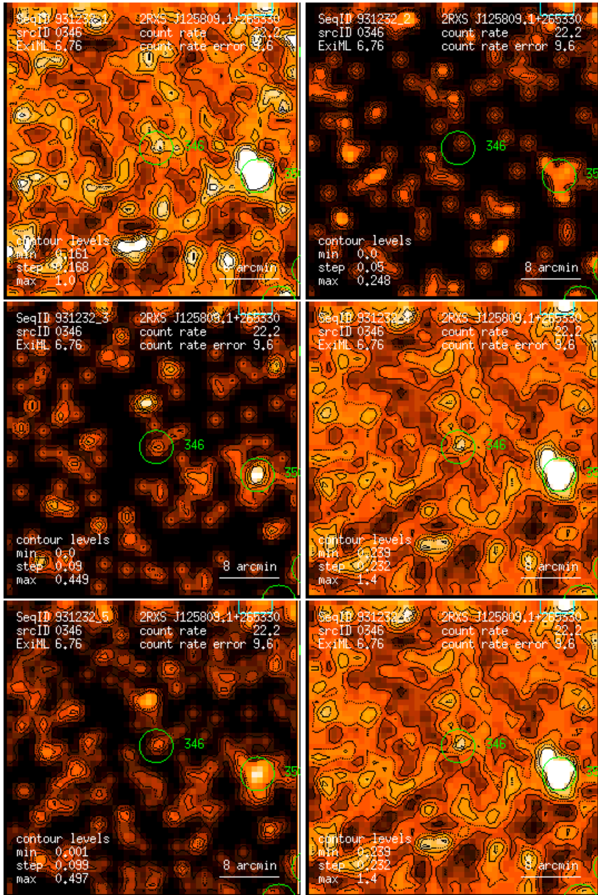
Figure 346: RASS 931232: detection 0346: band rate images, Gaussian filter: (1) PSPC channels 11 – 41, (2) 52 – 90, (3) 91 – 201, (4) 11 – 235, (5) 52 – 201, (6) 11 – 201. Broad band rates in counts/ks. Band rate contour levels in counts/ks/arcmin 2 .
