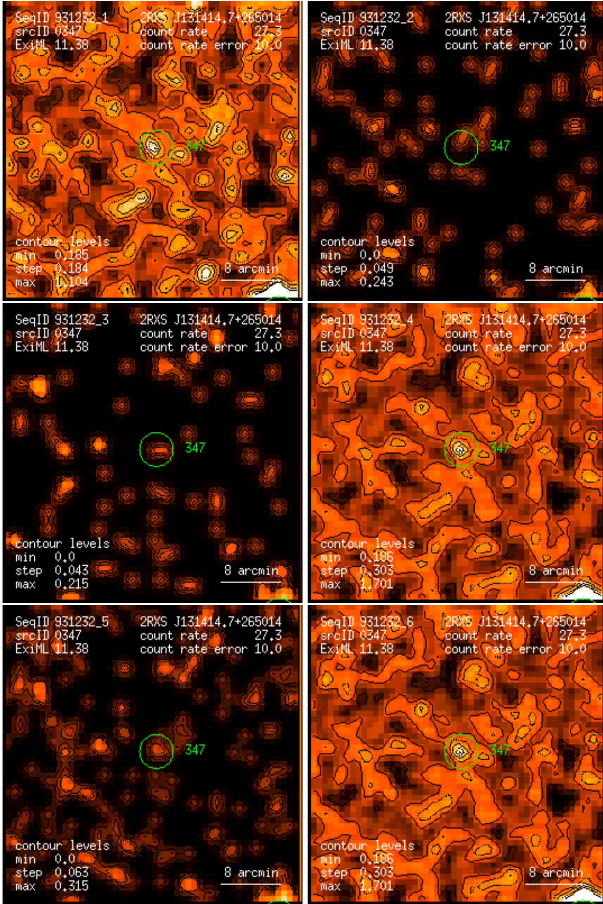
Figure 347: RASS 931232: detection 0347: band rate images, Gaussian filter: (1) PSPC channels 11 – 41, (2) 52 – 90, (3) 91 – 201, (4) 11 – 235, (5) 52 – 201, (6) 11 – 201. Broad band rates in counts/ks. Band rate contour levels in counts/ks/arcmin 2 .
