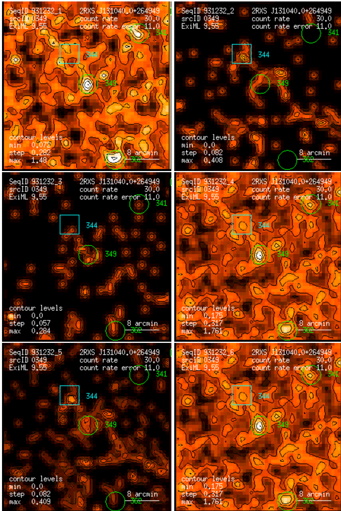
Figure 349: RASS 931232: detection 0349: band rate images, Gaussian filter: (1) PSPC channels 11 – 41, (2) 52 – 90, (3) 91 – 201, (4) 11 – 235, (5) 52 – 201, (6) 11 – 201. Broad band rates in counts/ks. Band rate contour levels in counts/ks/arcmin 2 .
