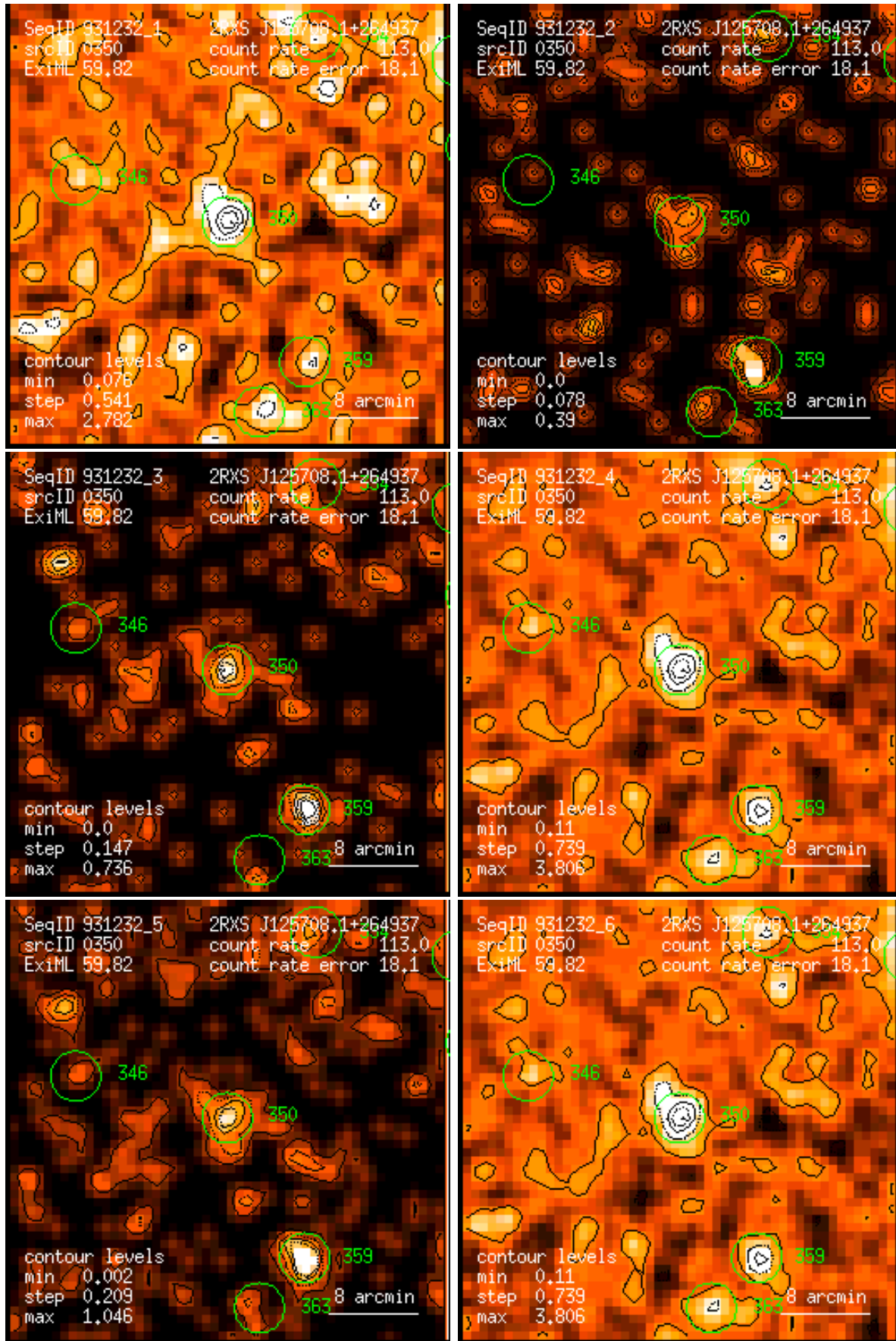
Figure 350: RASS 931232: detection 0350: band rate images, Gaussian filter: (1) PSPC channels 11 – 41, (2) 52 – 90, (3) 91 – 201, (4) 11 – 235, (5) 52 – 201, (6) 11 – 201. Broad band rates in counts/ks. Band rate contour levels in counts/ks/arcmin 2 .
