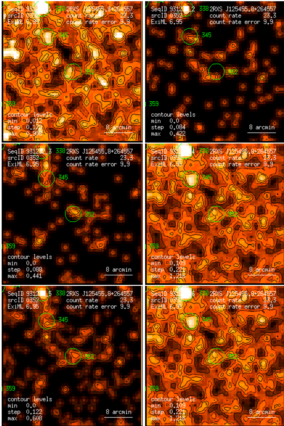
Figure 352: RASS 931232: detection 0352: band rate images, Gaussian filter: (1) PSPC channels 11 – 41, (2) 52 – 90, (3) 91 – 201, (4) 11 – 235, (5) 52 – 201, (6) 11 – 201. Broad band rates in counts/ks. Band rate contour levels in counts/ks/arcmin 2 .
