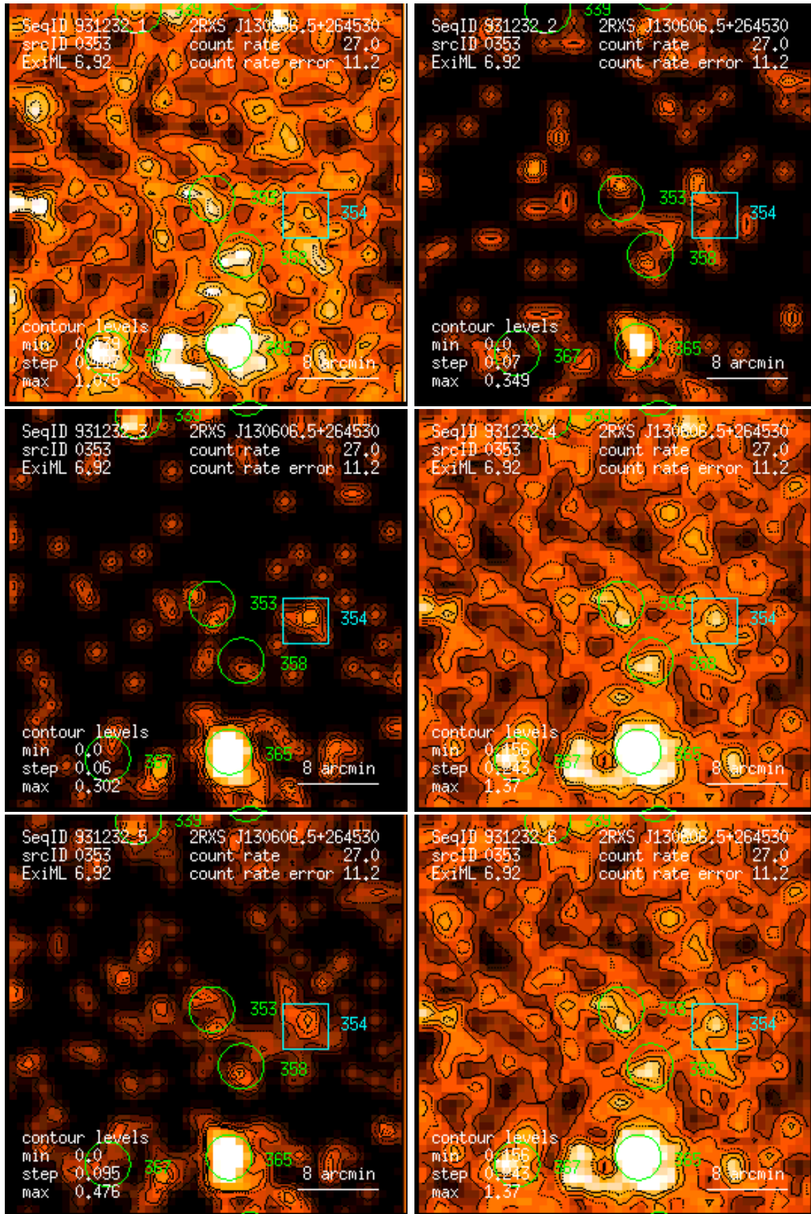
Figure 353: RASS 931232: detection 0353: band rate images, Gaussian filter: (1) PSPC channels 11 – 41, (2) 52 – 90, (3) 91 – 201, (4) 11 – 235, (5) 52 – 201, (6) 11 – 201. Broad band rates in counts/ks. Band rate contour levels in counts/ks/arcmin 2 .
