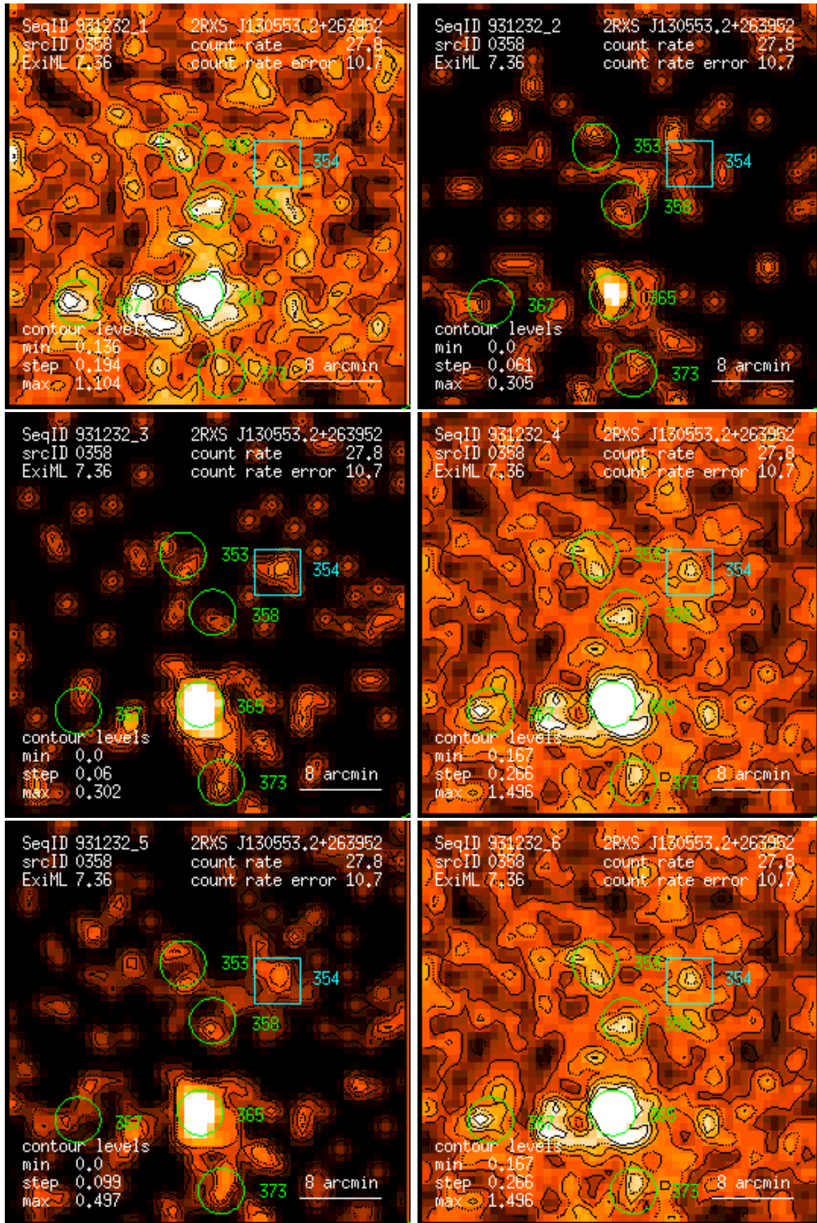
Figure 358: RASS 931232: detection 0358: band rate images, Gaussian filter: (1) PSPC channels 11 – 41, (2) 52 – 90, (3) 91 – 201, (4) 11 – 235, (5) 52 – 201, (6) 11 – 201. Broad band rates in counts/ks. Band rate contour levels in counts/ks/arcmin 2 .
