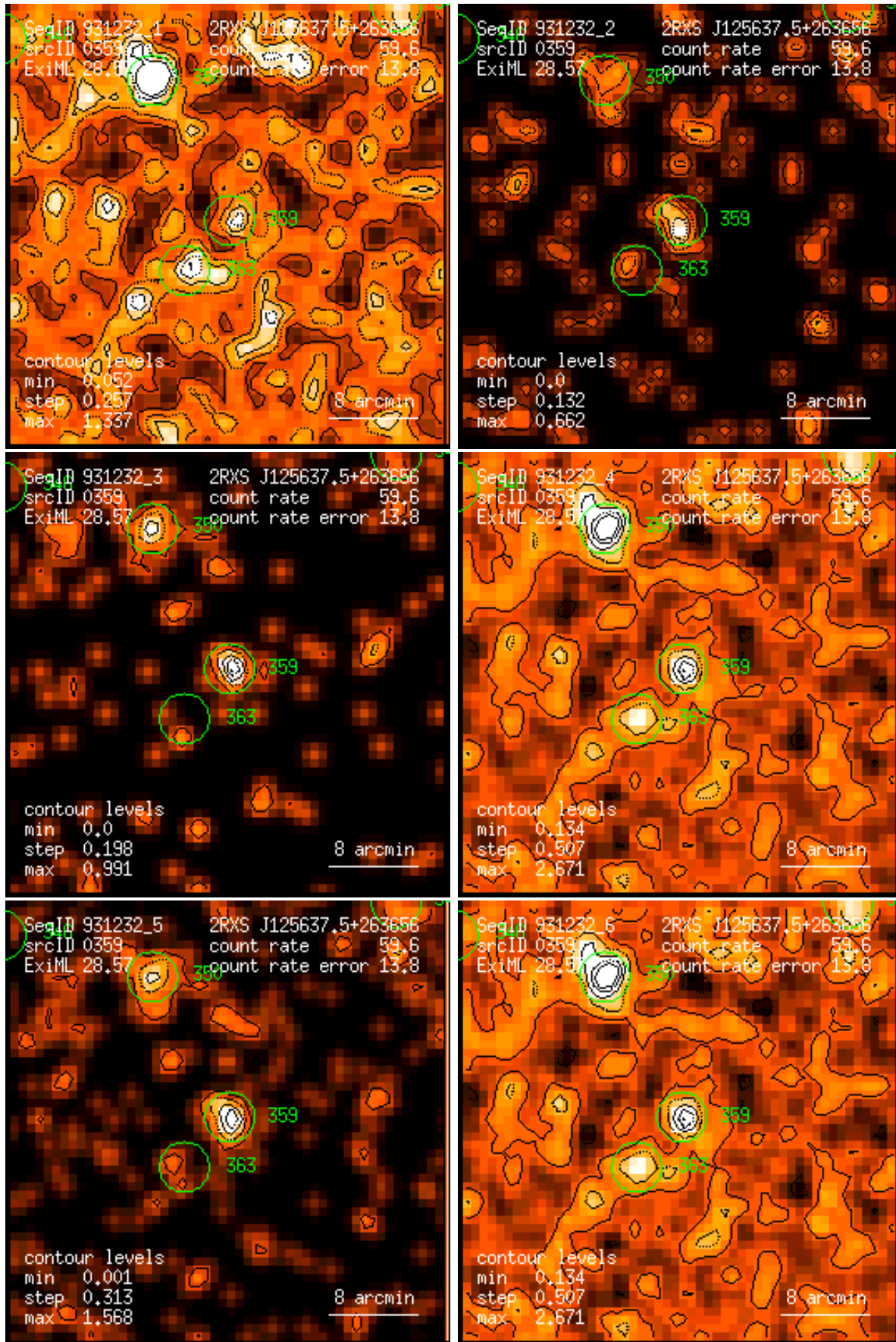
Figure 359: RASS 931232: detection 0359: band rate images, Gaussian filter: (1) PSPC channels 11 – 41, (2) 52 – 90, (3) 91 – 201, (4) 11 – 235, (5) 52 – 201, (6) 11 – 201. Broad band rates in counts/ks. Band rate contour levels in counts/ks/arcmin 2 .
