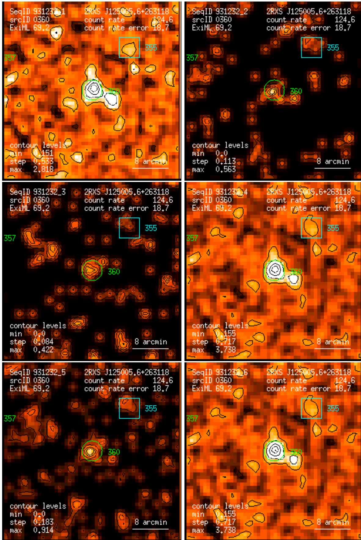
Figure 360: RASS 931232: detection 0360: band rate images, Gaussian filter: (1) PSPC channels 11 – 41, (2) 52 – 90, (3) 91 – 201, (4) 11 – 235, (5) 52 – 201, (6) 11 – 201. Broad band rates in counts/ks. Band rate contour levels in counts/ks/arcmin 2 .
