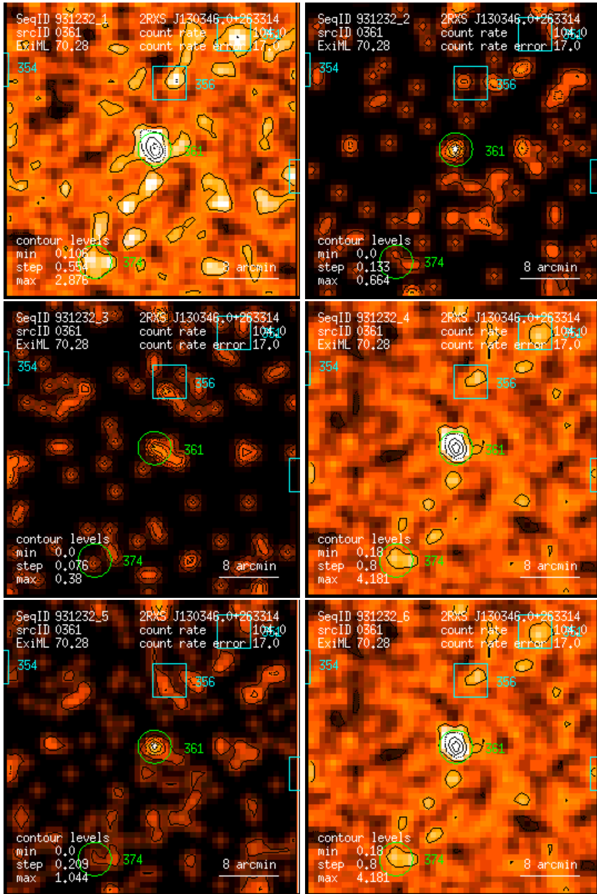
Figure 361: RASS 931232: detection 0361: band rate images, Gaussian filter: (1) PSPC channels 11 – 41, (2) 52 – 90, (3) 91 – 201, (4) 11 – 235, (5) 52 – 201, (6) 11 – 201. Broad band rates in counts/ks. Band rate contour levels in counts/ks/arcmin 2 .
