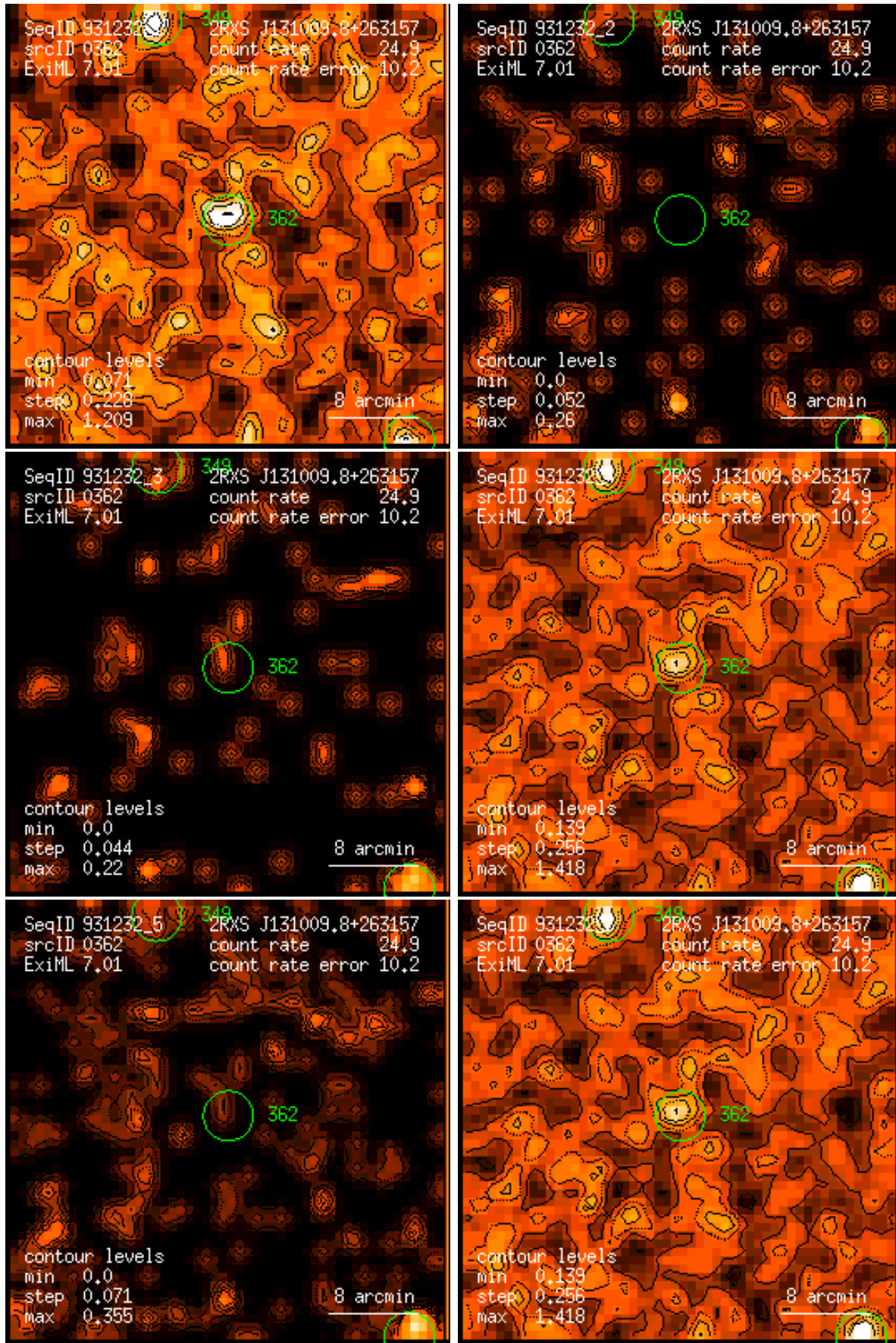
Figure 362: RASS 931232: detection 0362: band rate images, Gaussian filter: (1) PSPC channels 11 – 41, (2) 52 – 90, (3) 91 – 201, (4) 11 – 235, (5) 52 – 201, (6) 11 – 201. Broad band rates in counts/ks. Band rate contour levels in counts/ks/arcmin 2 .
