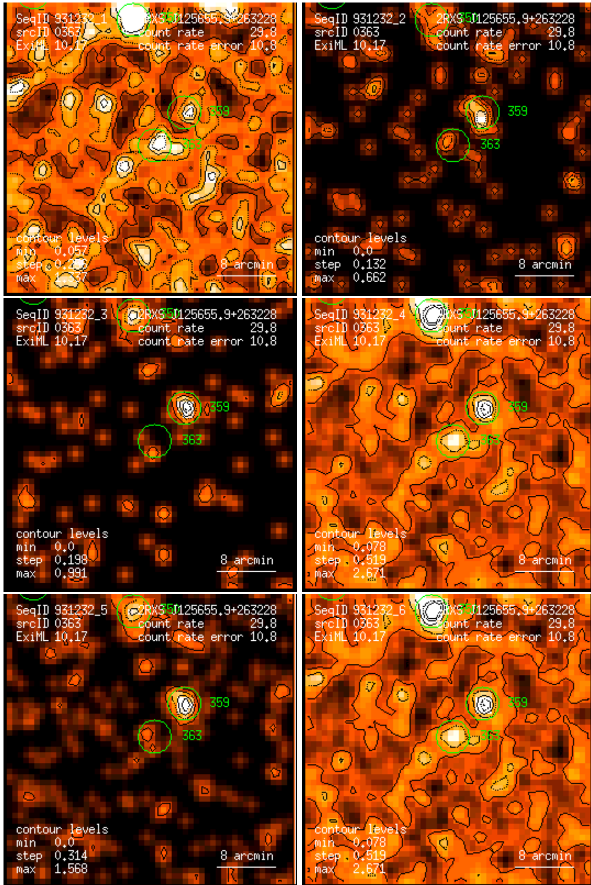
Figure 363: RASS 931232: detection 0363: band rate images, Gaussian filter: (1) PSPC channels 11 – 41, (2) 52 – 90, (3) 91 – 201, (4) 11 – 235, (5) 52 – 201, (6) 11 – 201. Broad band rates in counts/ks. Band rate contour levels in counts/ks/arcmin 2 .
