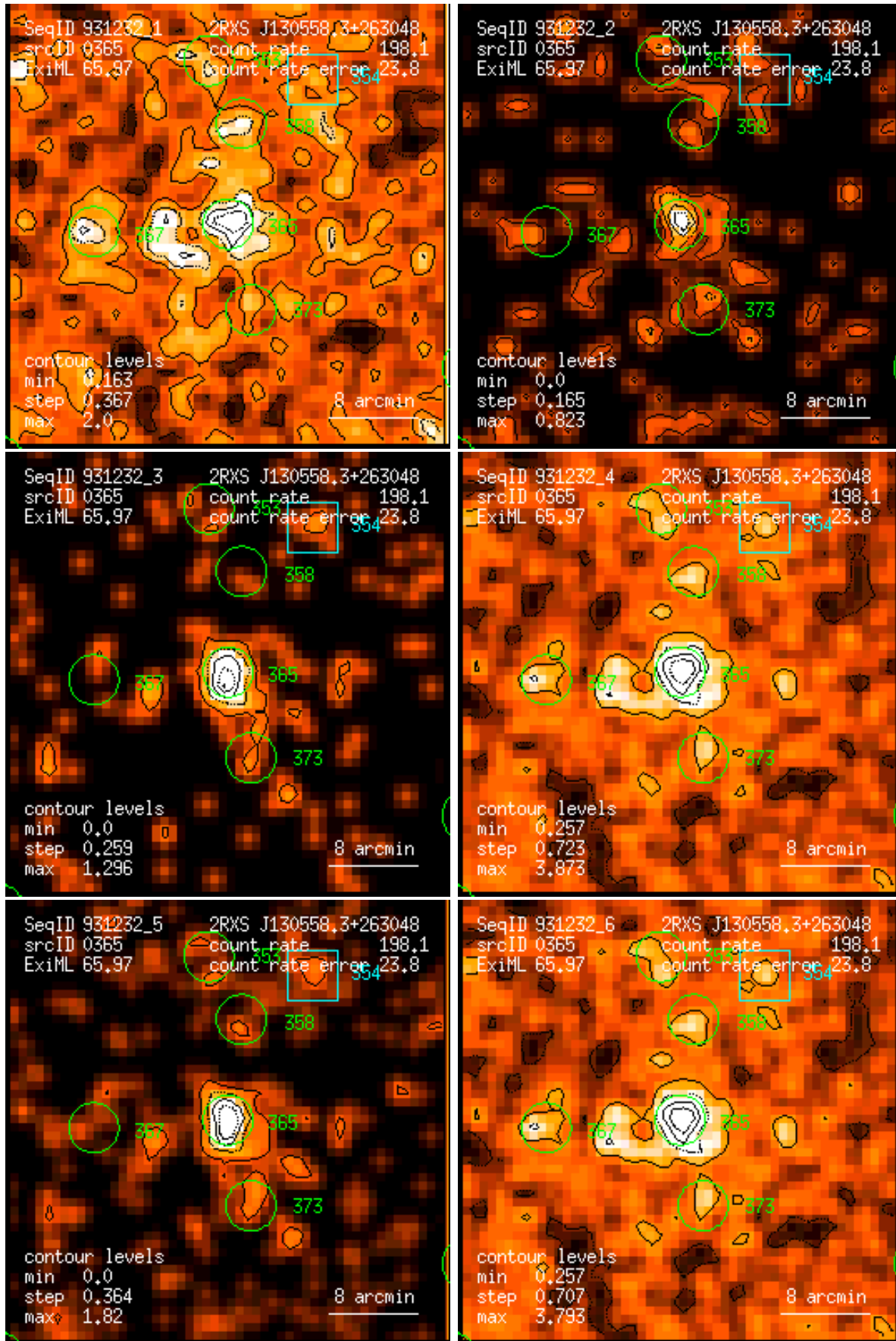
Figure 365: RASS 931232: detection 0365: band rate images, Gaussian filter: (1) PSPC channels 11 – 41, (2) 52 – 90, (3) 91 – 201, (4) 11 – 235, (5) 52 – 201, (6) 11 – 201. Broad band rates in counts/ks. Band rate contour levels in counts/ks/arcmin 2 .
