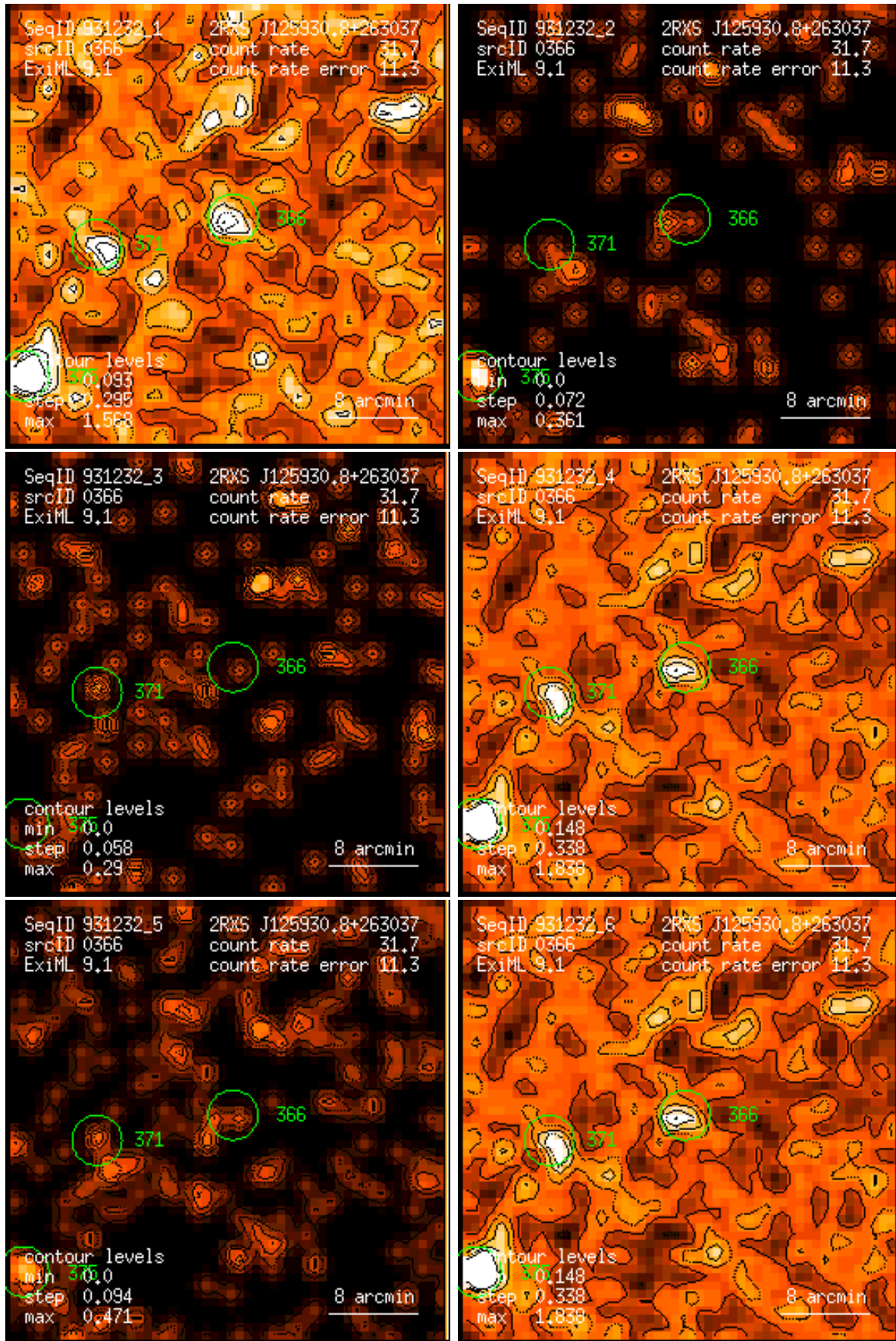
Figure 366: RASS 931232: detection 0366: band rate images, Gaussian filter: (1) PSPC channels 11 – 41, (2) 52 – 90, (3) 91 – 201, (4) 11 – 235, (5) 52 – 201, (6) 11 – 201. Broad band rates in counts/ks. Band rate contour levels in counts/ks/arcmin 2 .
