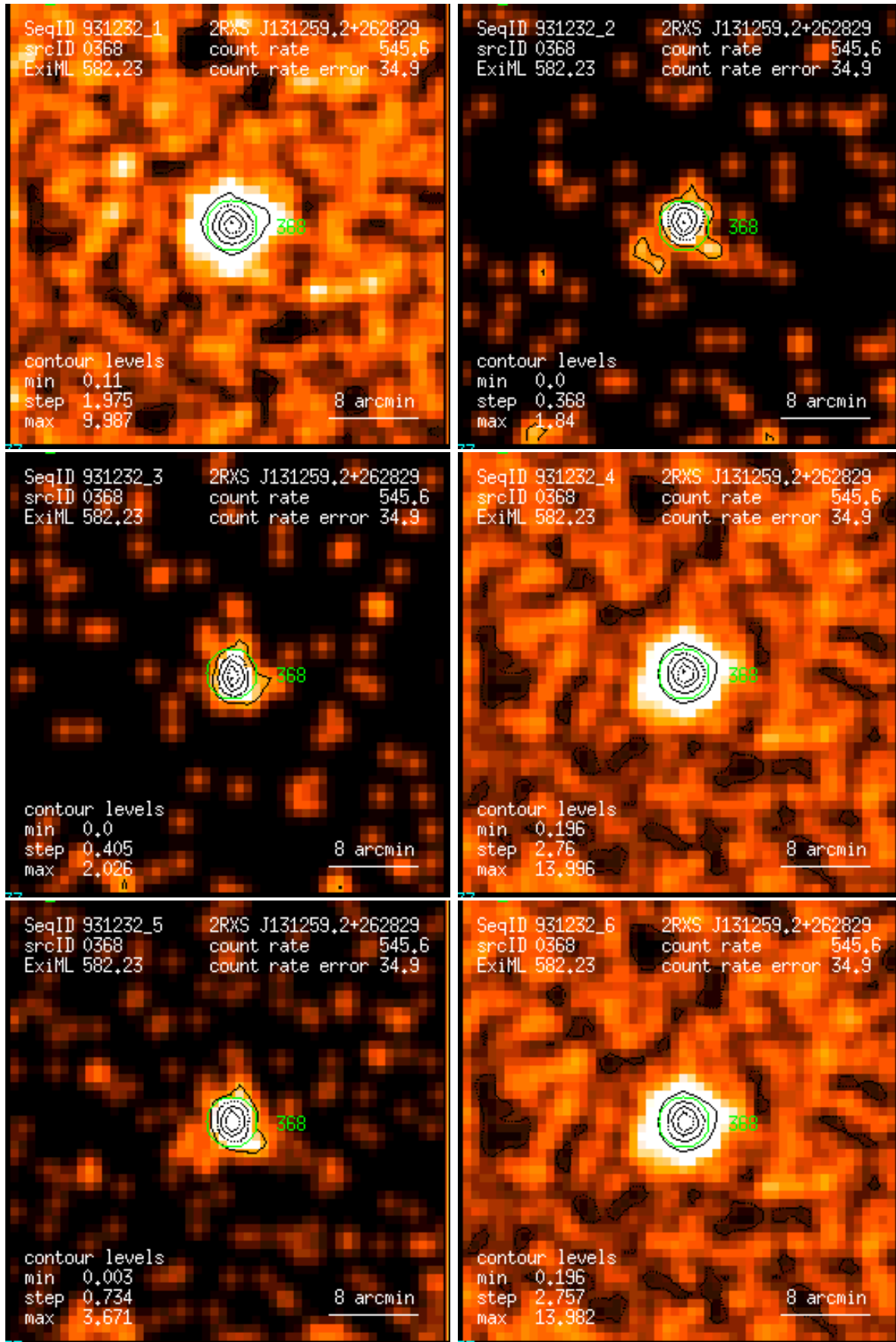
Figure 368: RASS 931232: detection 0368: band rate images, Gaussian filter: (1) PSPC channels 11 – 41, (2) 52 – 90, (3) 91 – 201, (4) 11 – 235, (5) 52 – 201, (6) 11 – 201. Broad band rates in counts/ks. Band rate contour levels in counts/ks/arcmin 2 .
