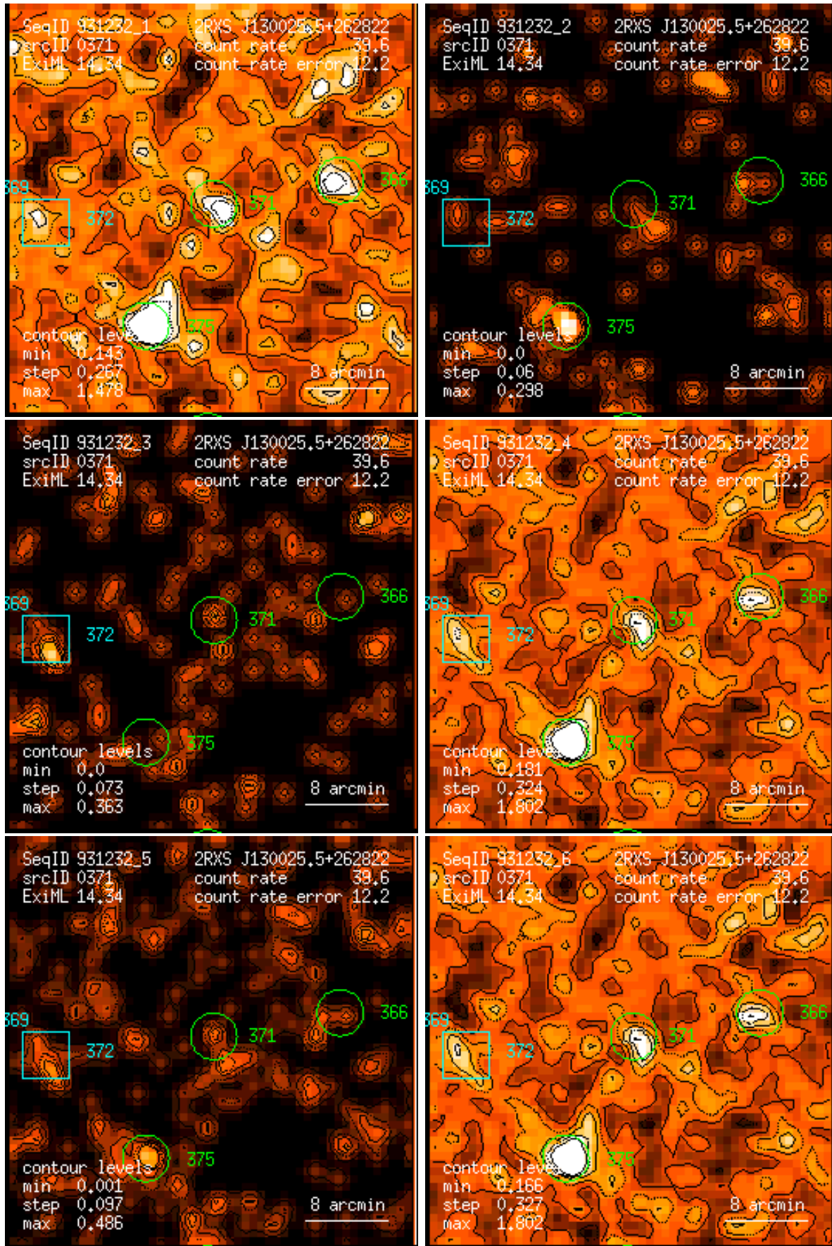
Figure 371: RASS 931232: detection 0371: band rate images, Gaussian filter: (1) PSPC channels 11 – 41, (2) 52 – 90, (3) 91 – 201, (4) 11 – 235, (5) 52 – 201, (6) 11 – 201. Broad band rates in counts/ks. Band rate contour levels in counts/ks/arcmin 2 .
