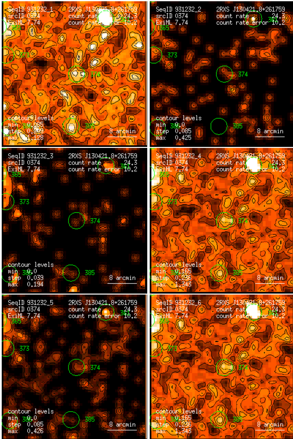
Figure 374: RASS 931232: detection 0374: band rate images, Gaussian filter: (1) PSPC channels 11 – 41, (2) 52 – 90, (3) 91 – 201, (4) 11 – 235, (5) 52 – 201, (6) 11 – 201. Broad band rates in counts/ks. Band rate contour levels in counts/ks/arcmin 2 .
