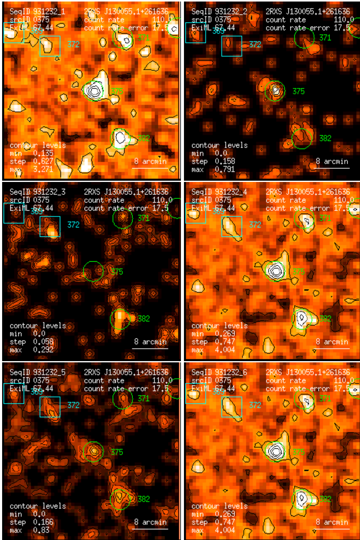
Figure 375: RASS 931232: detection 0375: band rate images, Gaussian filter: (1) PSPC channels 11 – 41, (2) 52 – 90, (3) 91 – 201, (4) 11 – 235, (5) 52 – 201, (6) 11 – 201. Broad band rates in counts/ks. Band rate contour levels in counts/ks/arcmin 2 .
