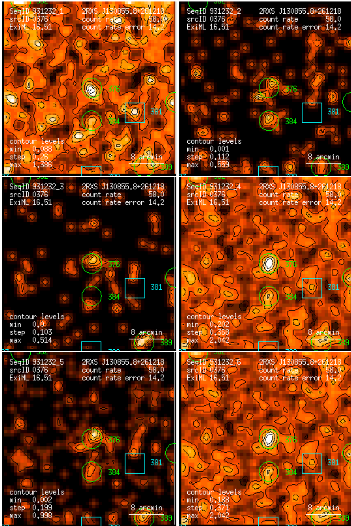
Figure 376: RASS 931232: detection 0376: band rate images, Gaussian filter: (1) PSPC channels 11 – 41, (2) 52 – 90, (3) 91 – 201, (4) 11 – 235, (5) 52 – 201, (6) 11 – 201. Broad band rates in counts/ks. Band rate contour levels in counts/ks/arcmin 2 .
