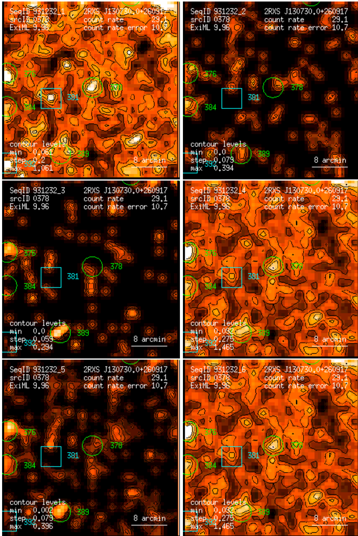
Figure 378: RASS 931232: detection 0378: band rate images, Gaussian filter: (1) PSPC channels 11 – 41, (2) 52 – 90, (3) 91 – 201, (4) 11 – 235, (5) 52 – 201, (6) 11 – 201. Broad band rates in counts/ks. Band rate contour levels in counts/ks/arcmin 2 .
