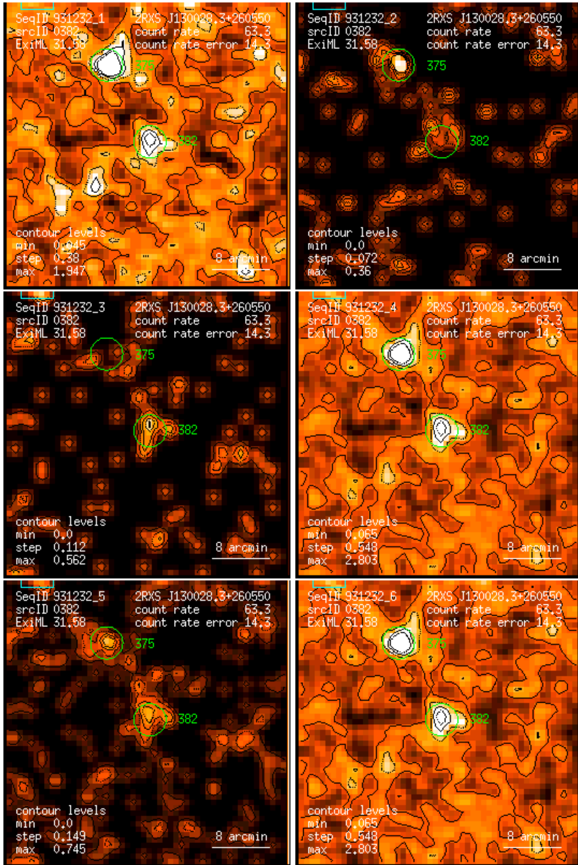
Figure 382: RASS 931232: detection 0382: band rate images, Gaussian filter: (1) PSPC channels 11 – 41, (2) 52 – 90, (3) 91 – 201, (4) 11 – 235, (5) 52 – 201, (6) 11 – 201. Broad band rates in counts/ks. Band rate contour levels in counts/ks/arcmin 2 .
