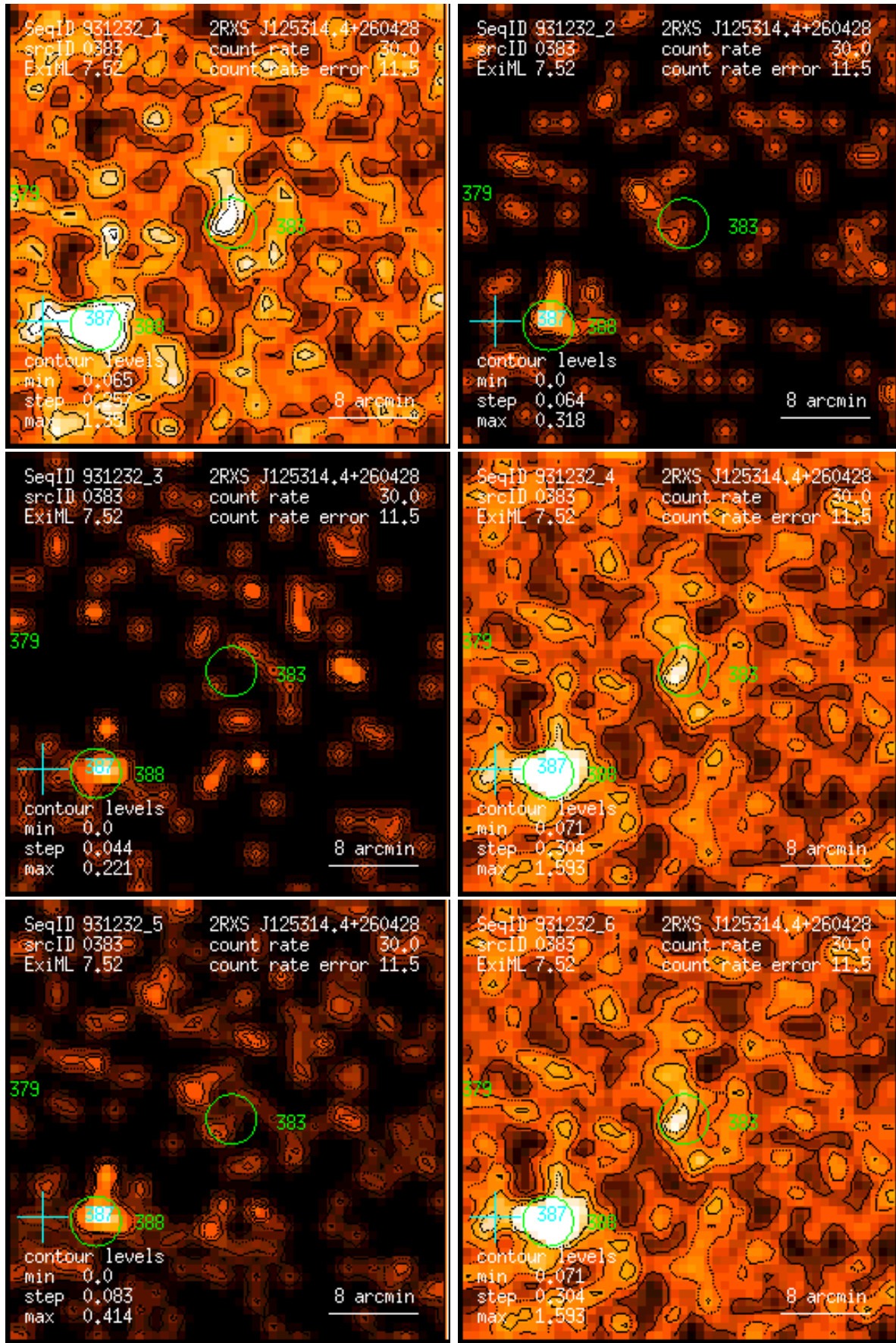
Figure 383: RASS 931232: detection 0383: band rate images, Gaussian filter: (1) PSPC channels 11 – 41, (2) 52 – 90, (3) 91 – 201, (4) 11 – 235, (5) 52 – 201, (6) 11 – 201. Broad band rates in counts/ks. Band rate contour levels in counts/ks/arcmin 2 .
