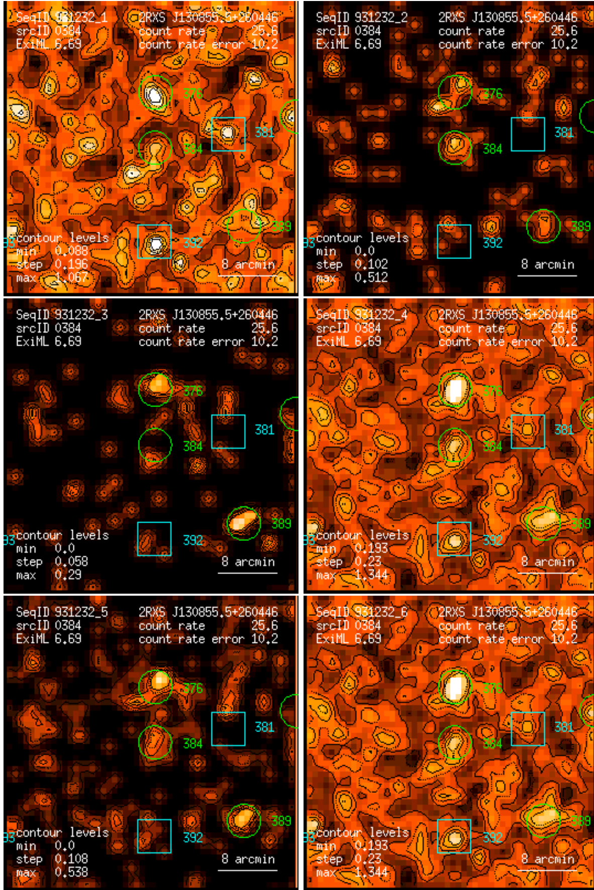
Figure 384: RASS 931232: detection 0384: band rate images, Gaussian filter: (1) PSPC channels 11 – 41, (2) 52 – 90, (3) 91 – 201, (4) 11 – 235, (5) 52 – 201, (6) 11 – 201. Broad band rates in counts/ks. Band rate contour levels in counts/ks/arcmin 2 .
