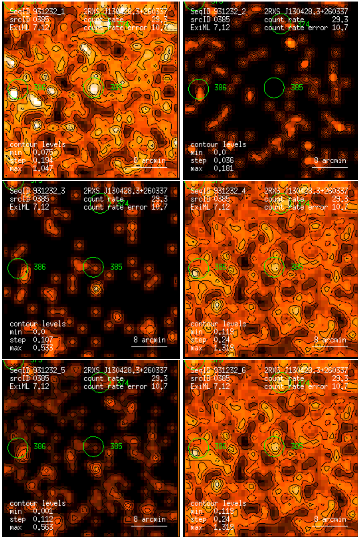
Figure 385: RASS 931232: detection 0385: band rate images, Gaussian filter: (1) PSPC channels 11 – 41, (2) 52 – 90, (3) 91 – 201, (4) 11 – 235, (5) 52 – 201, (6) 11 – 201. Broad band rates in counts/ks. Band rate contour levels in counts/ks/arcmin 2 .
