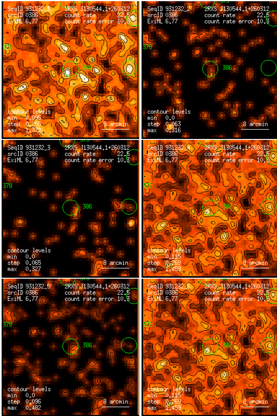
Figure 386: RASS 931232: detection 0386: band rate images, Gaussian filter: (1) PSPC channels 11 – 41, (2) 52 – 90, (3) 91 – 201, (4) 11 – 235, (5) 52 – 201, (6) 11 – 201. Broad band rates in counts/ks. Band rate contour levels in counts/ks/arcmin 2 .
