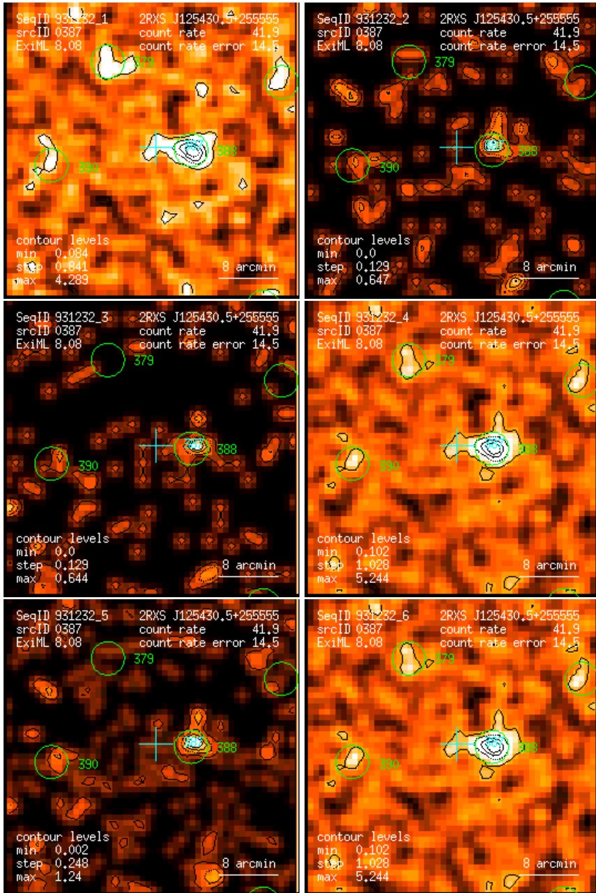
Figure 387: RASS 931232: detection 0387: band rate images, Gaussian filter: (1) PSPC channels 11 – 41, (2) 52 – 90, (3) 91 – 201, (4) 11 – 235, (5) 52 – 201, (6) 11 – 201. Broad band rates in counts/ks. Band rate contour levels in counts/ks/arcmin 2 .
