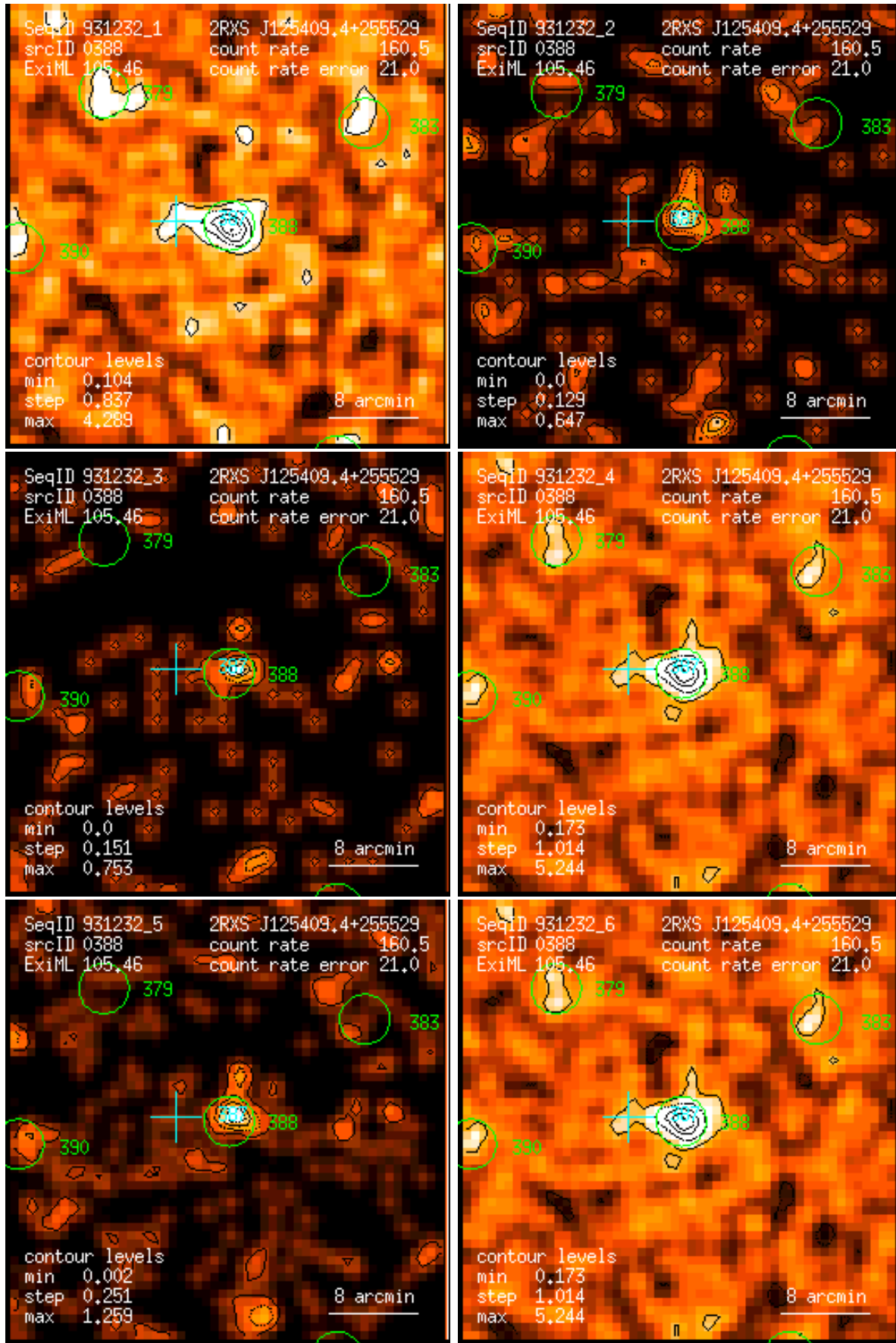
Figure 388: RASS 931232: detection 0388: band rate images, Gaussian filter: (1) PSPC channels 11 – 41, (2) 52 – 90, (3) 91 – 201, (4) 11 – 235, (5) 52 – 201, (6) 11 – 201. Broad band rates in counts/ks. Band rate contour levels in counts/ks/arcmin 2 .
