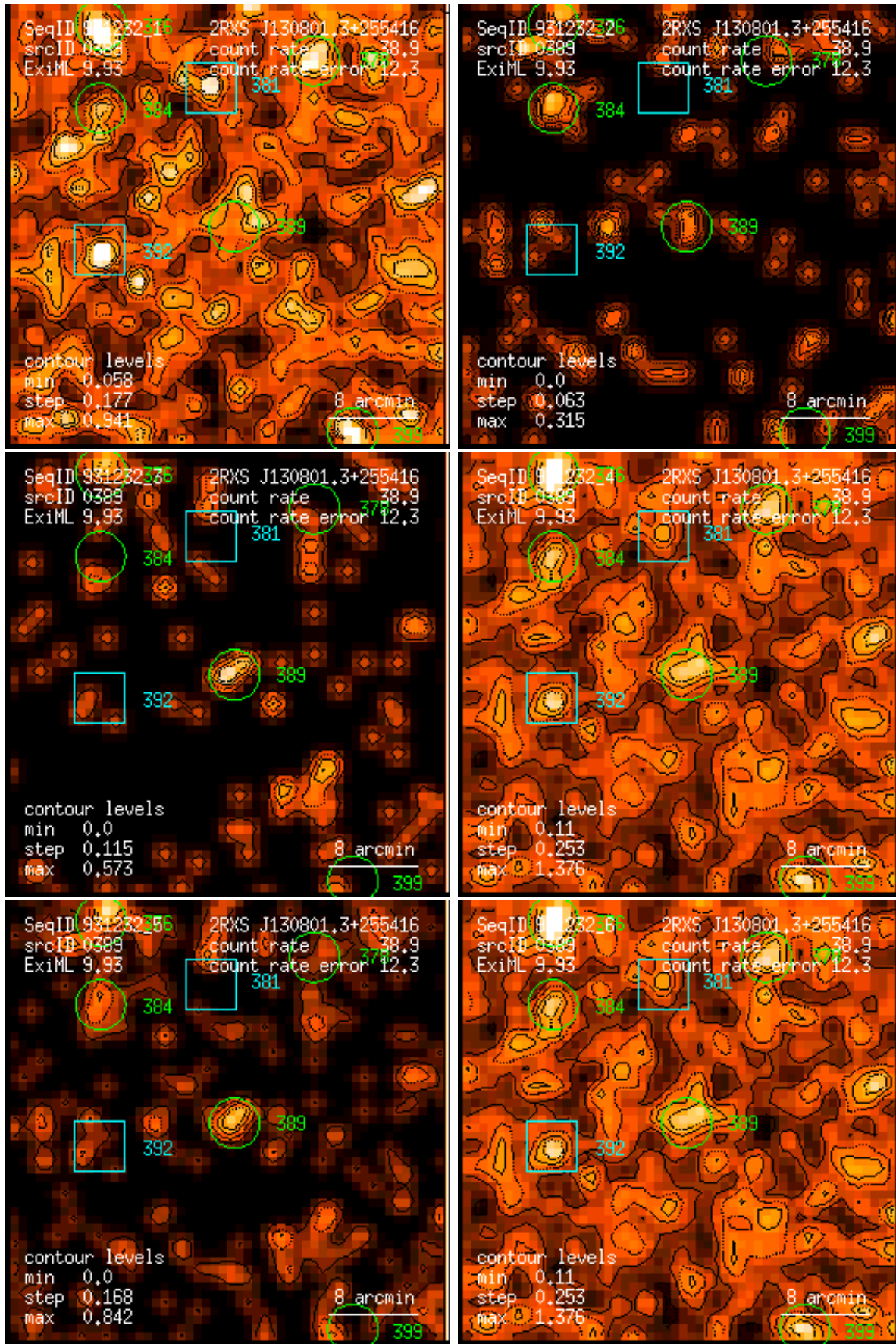
Figure 389: RASS 931232: detection 0389: band rate images, Gaussian filter: (1) PSPC channels 11 – 41, (2) 52 – 90, (3) 91 – 201, (4) 11 – 235, (5) 52 – 201, (6) 11 – 201. Broad band rates in counts/ks. Band rate contour levels in counts/ks/arcmin 2 .
