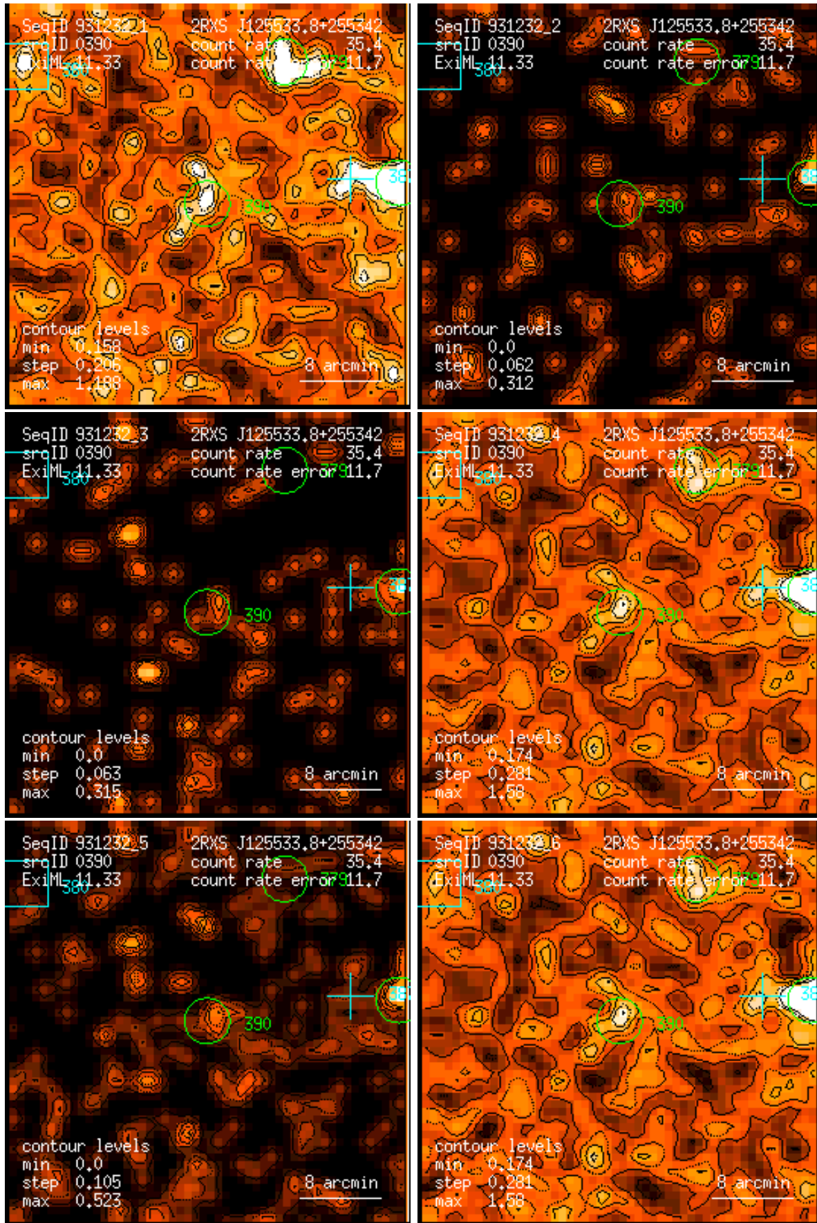
Figure 390: RASS 931232: detection 0390: band rate images, Gaussian filter: (1) PSPC channels 11 – 41, (2) 52 – 90, (3) 91 – 201, (4) 11 – 235, (5) 52 – 201, (6) 11 – 201. Broad band rates in counts/ks. Band rate contour levels in counts/ks/arcmin 2 .
